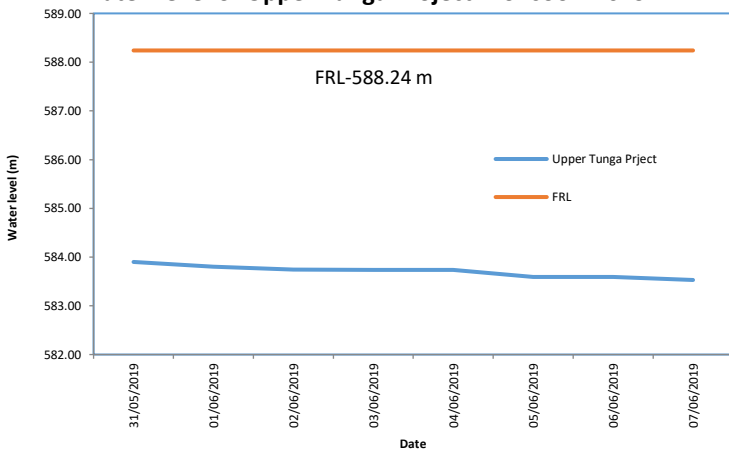
Water Level of Upper Tunga Project Monsoon-2019
