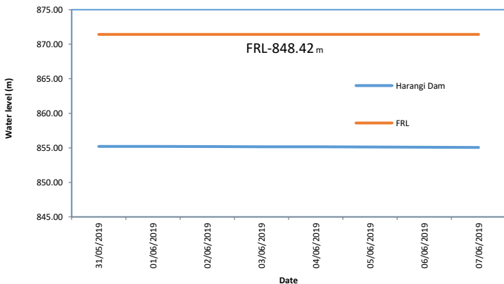
Water Level of Harangi Dam Monsoon-2019
