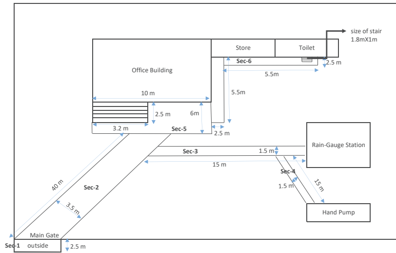
Drawing For Providing & fixing of INTERLOCKING PAVER BLOCK at Pali Site under LCSD, CWC, Jaipur
