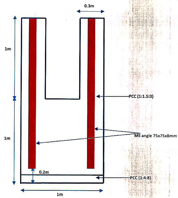
Front View of second supporting block
