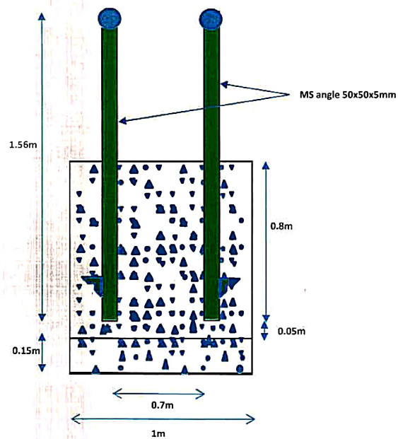
Section1-1
