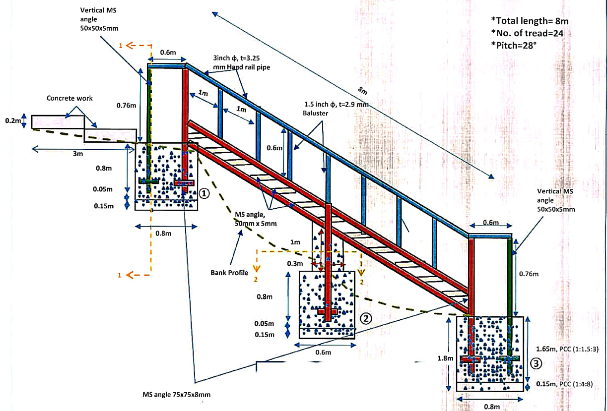
Drawing of Fabrication &amp; Installation of 8 meter M.S. Staircase at site Salebardi
