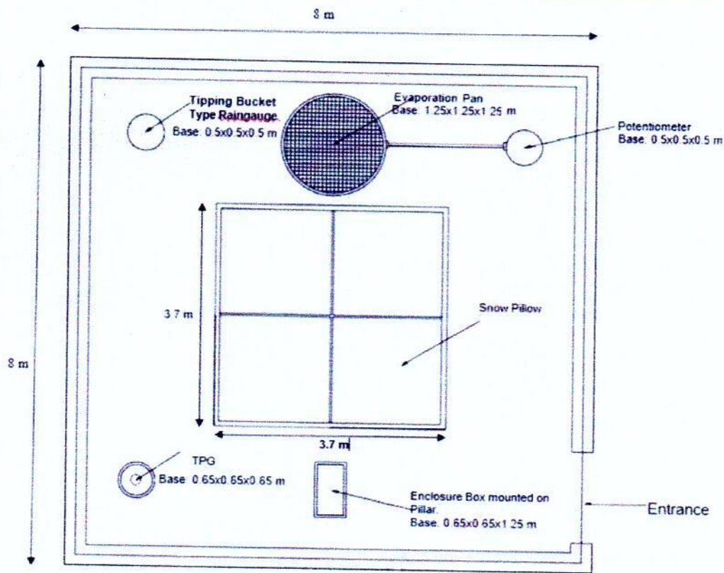
Layout Plan
