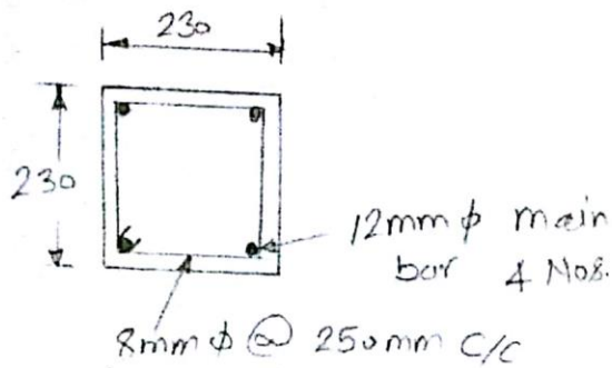
SECTION AT B-B
