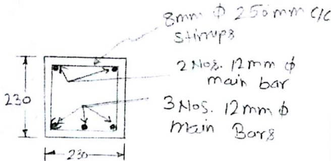
SECTION AT C-C
