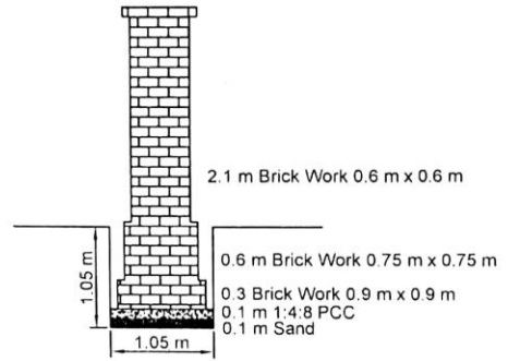
Sectional View of Gate Pillars
