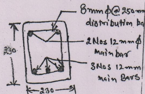
Section at C-C
