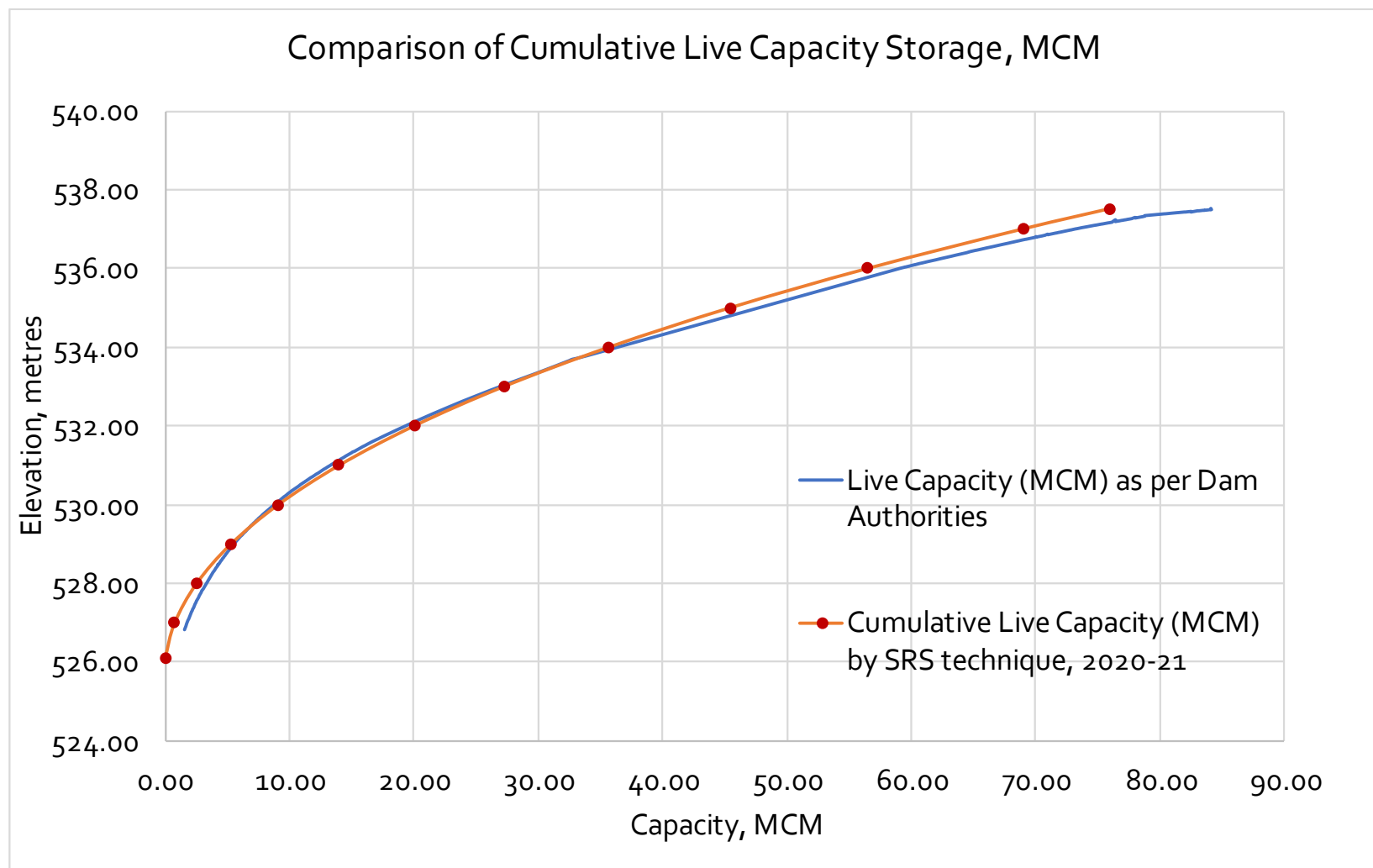
Figure 13: Comparison of Elevation - Live Storage Capacity curves (MCM) for Himayat Sagar Reservoir.
