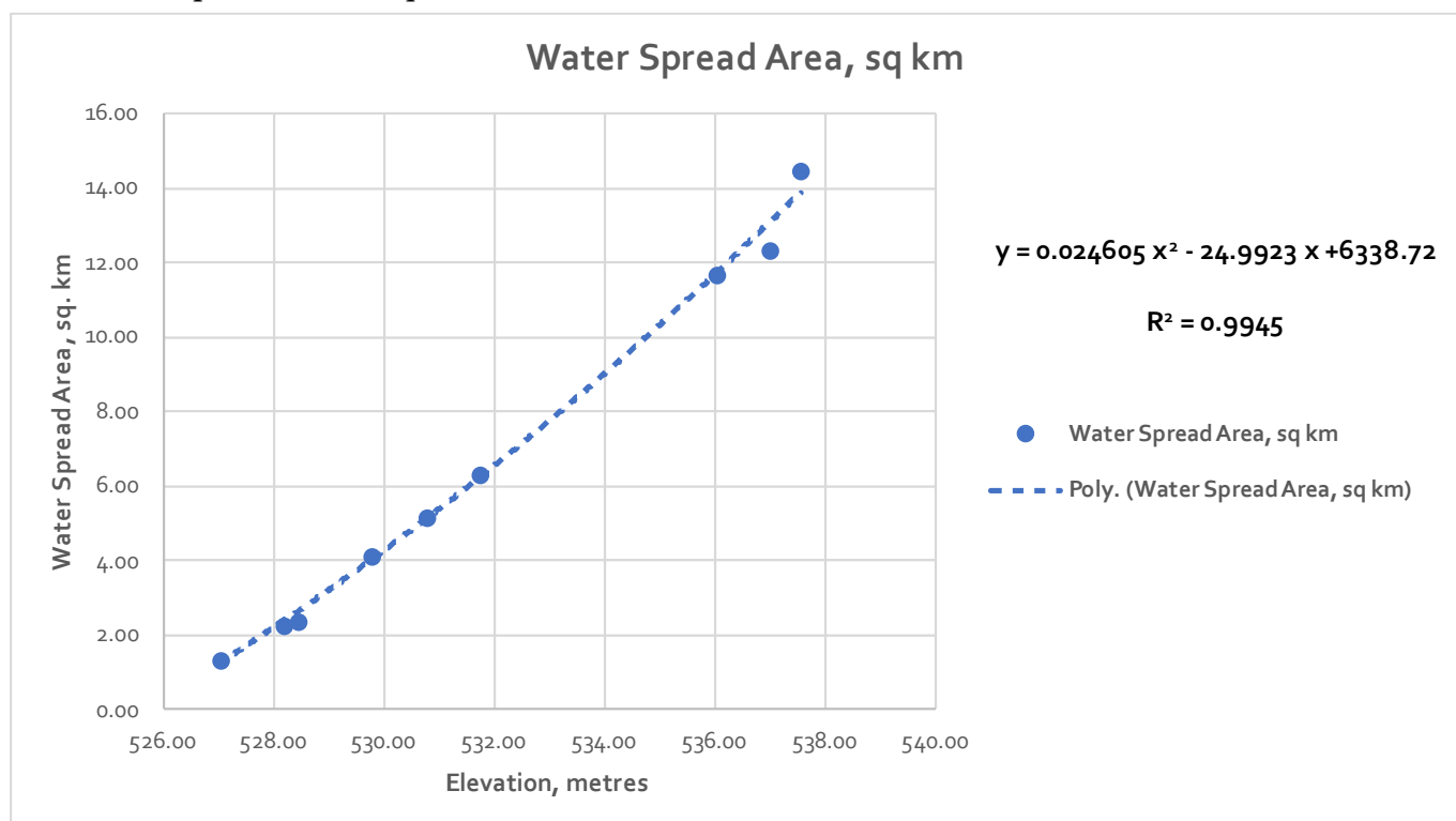
Figure 10: Observed Elevation vs. Observed Water Spread Area and Best Fit Curve for Himayat Sagar Reservoir.
