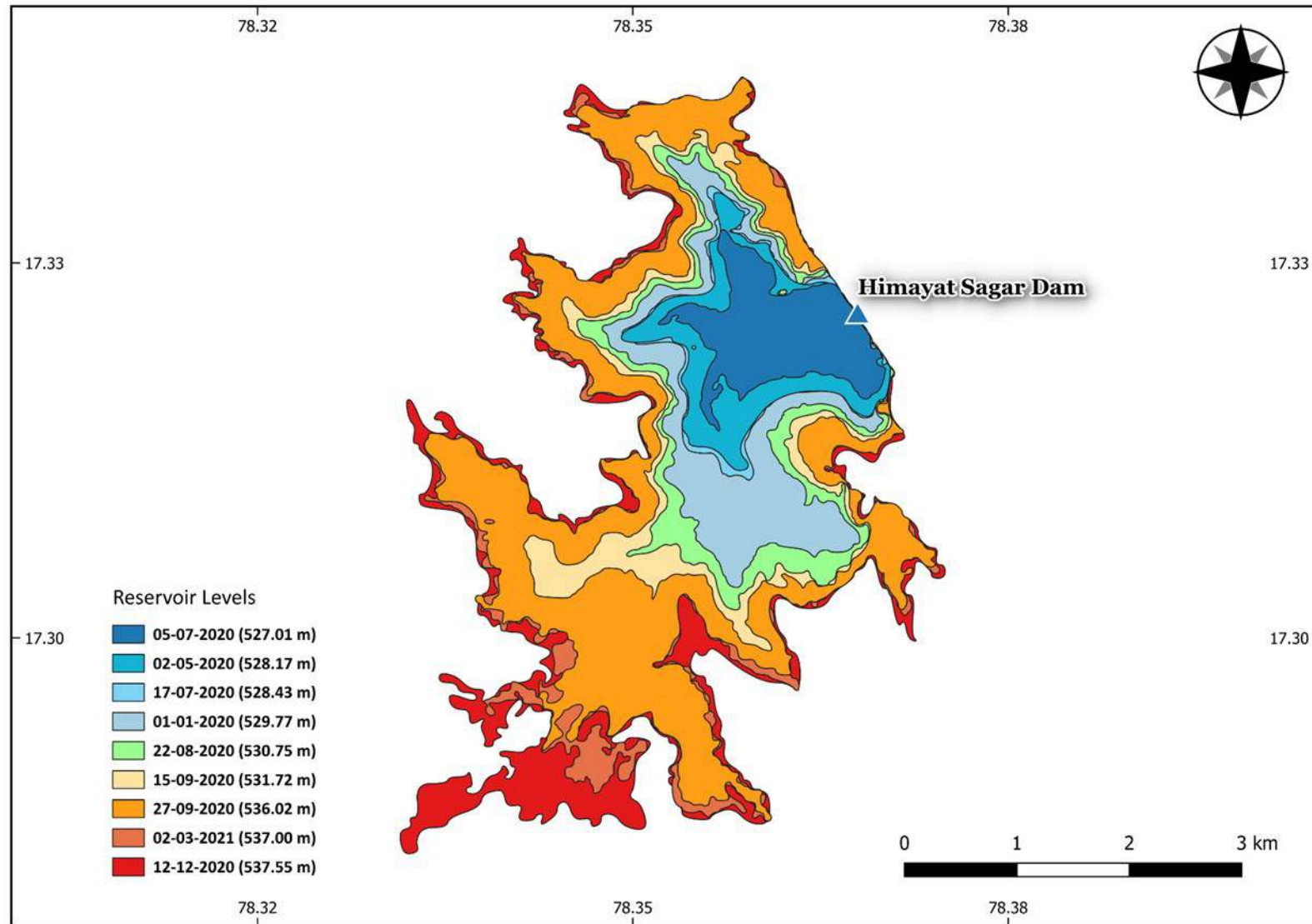
Figure 9: Water spread area at different levels of Himayat Sagar Reservoir.
