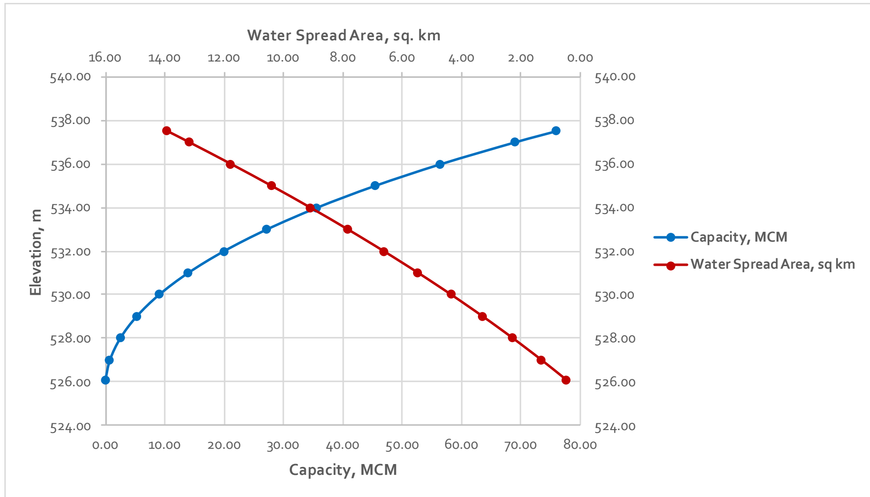
Figure 12: Elevation – Area – Capacity Curve for Himayat Sagar Reservoir.
