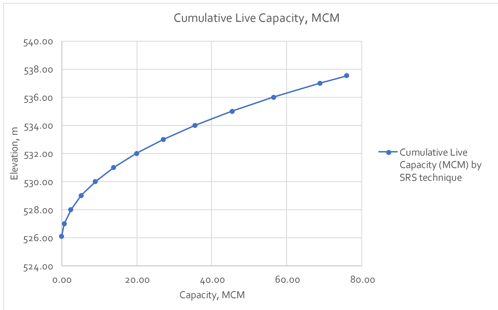
Figure 11: Modified live capacity - elevation curve (SRS technique) for Himayat Sagar Reservoir.
