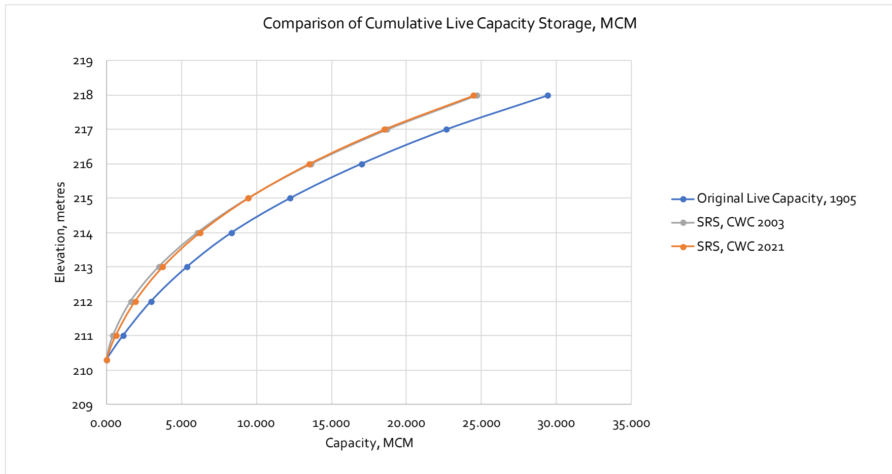
Figure 13: Comparison of Elevation - Live Storage Capacity curves (MCM) for Ram Sagar Reservoir.
