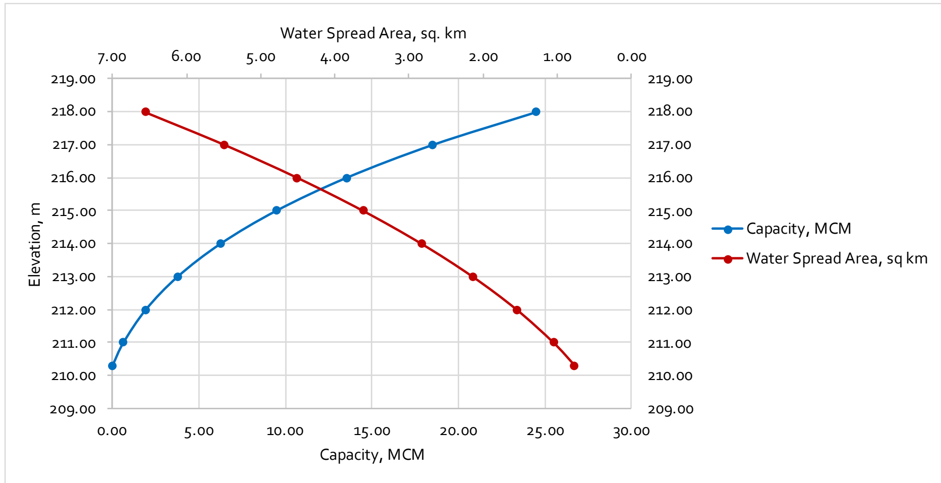
Figure 12: Elevation – Area – Capacity Curve for Ram Sagar Reservoir.
