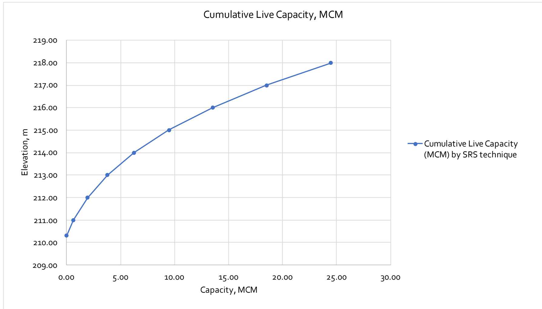
Figure 11: Modified live capacity - elevation curve (SRS technique) for Ram Sagar Reservoir.
