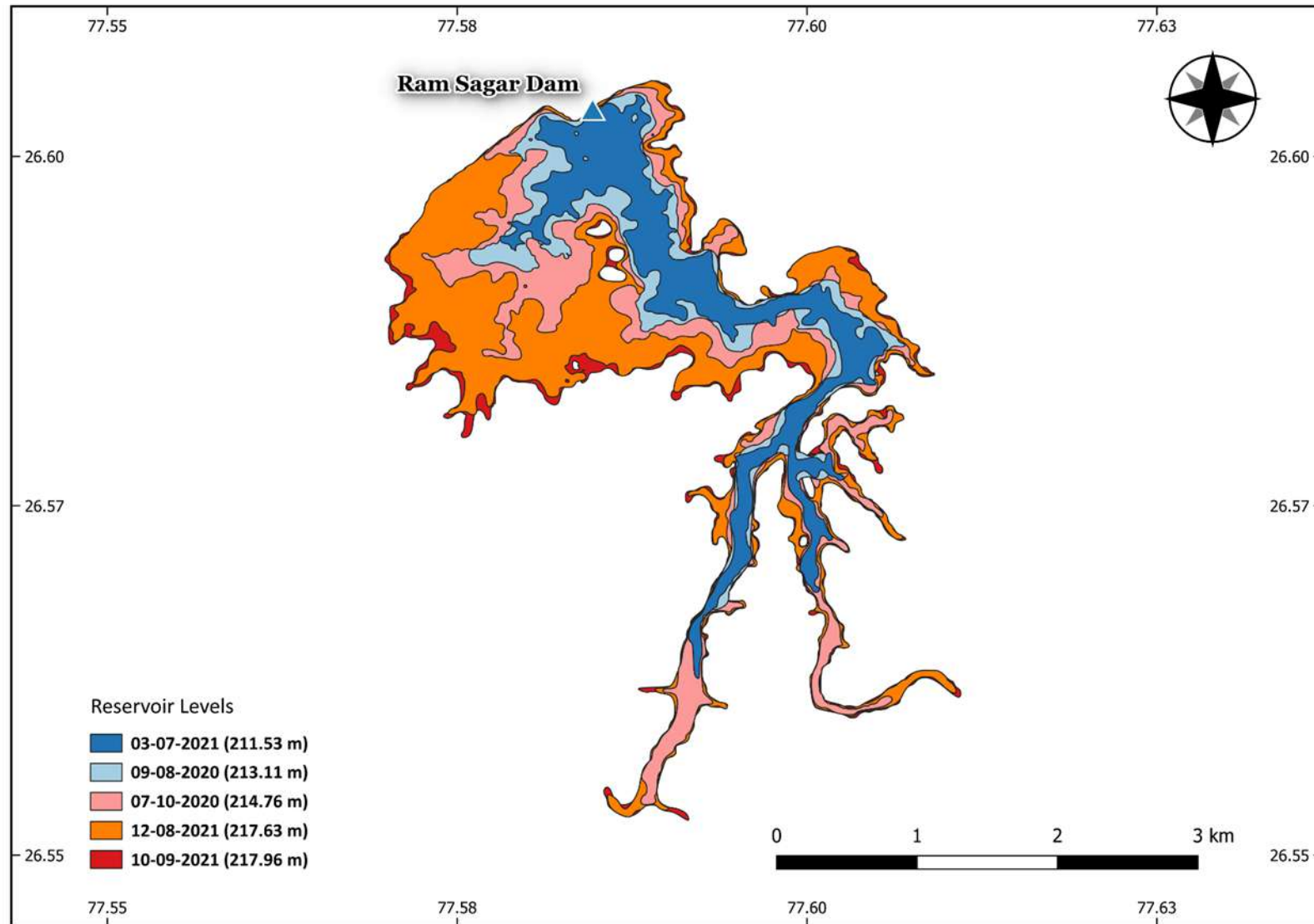
Figure 9: Water spread area at different levels of Ram Sagar Reservoir.
