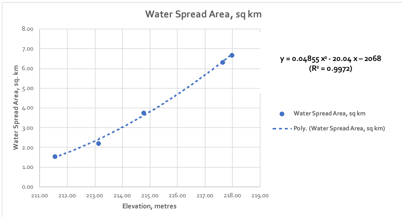
Figure 10: Observed Elevation vs. Observed Water Spread Area and Best Fit Curve for Ram Sagar Reservoir.
