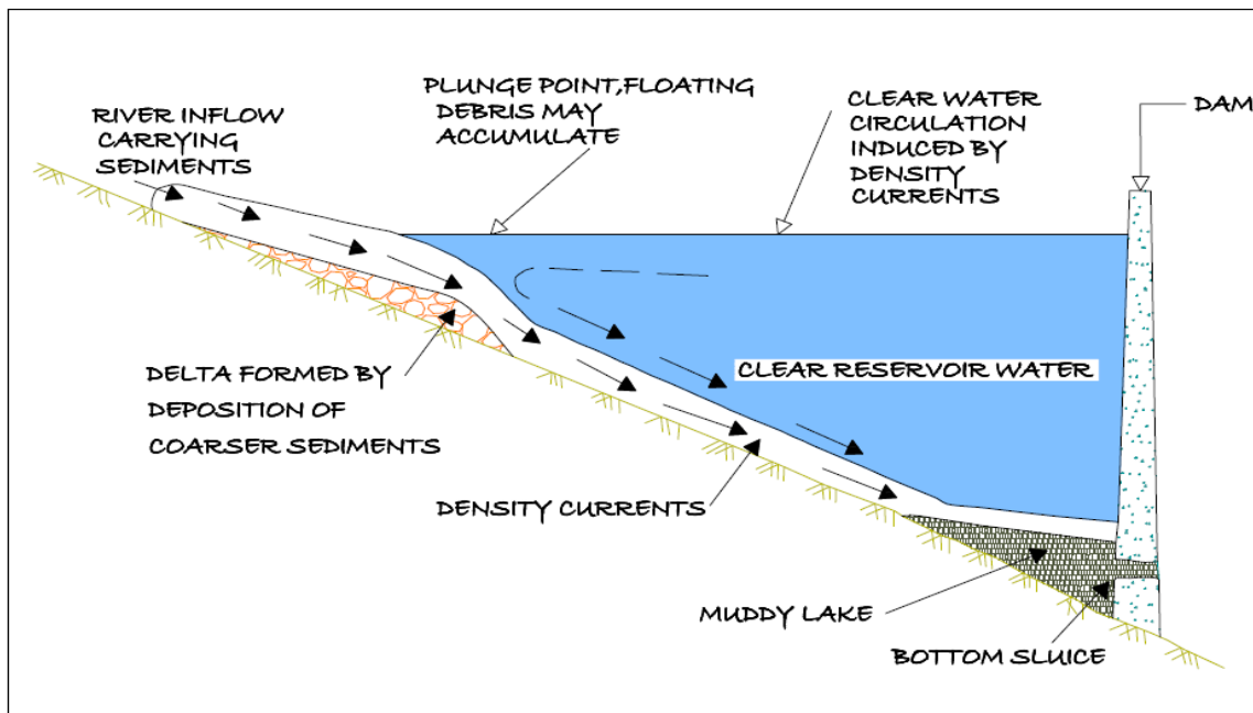
Fig. 1: Conceptual sketch of density currents in a reservoir
