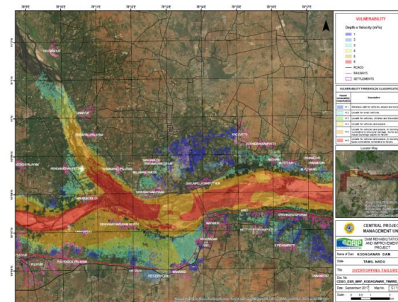
Figure 21 - An Inundation Map of Kodaganar Dam
