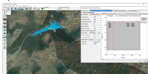
Figure 20 - DBA modeling process with HECRAS 2DH v5.0.3
