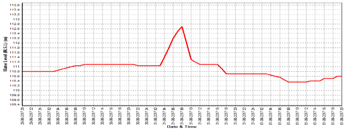
Water Level v/s Time graph of Highest (II) Flood Peak during the water year 2017-18
