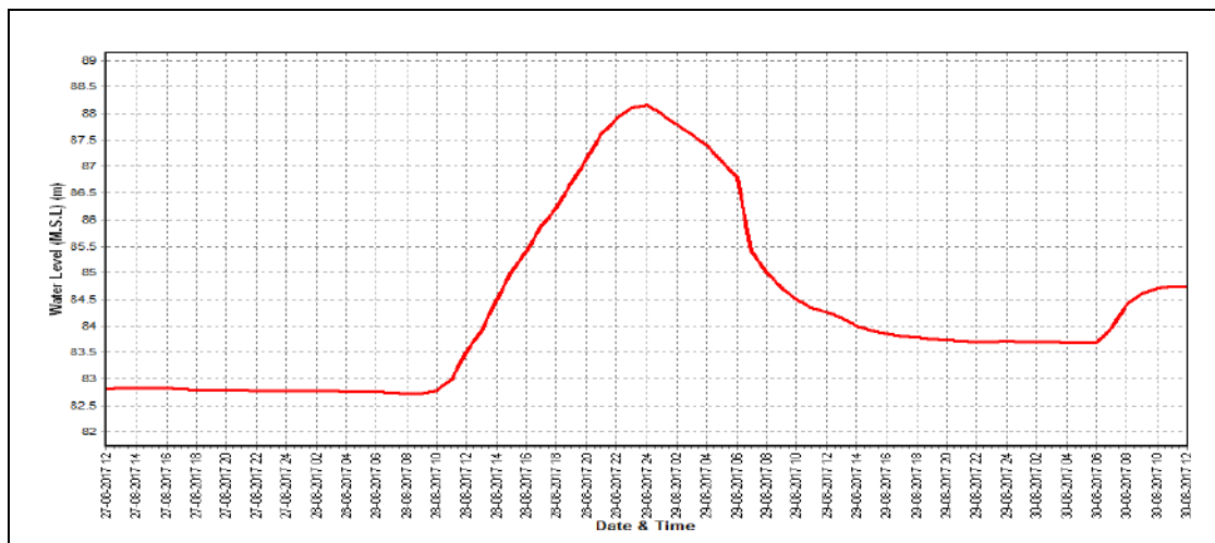
Water level vs. Time graph of III flood peak during the year 2017-18
