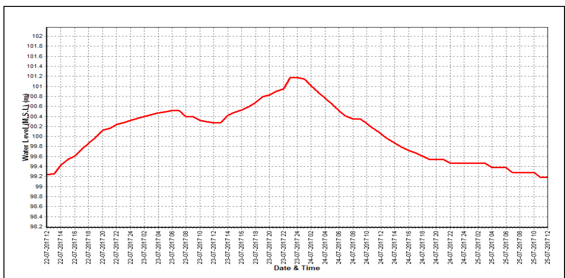
Water level vs. Time graph of III flood peak during the year 2017-18
