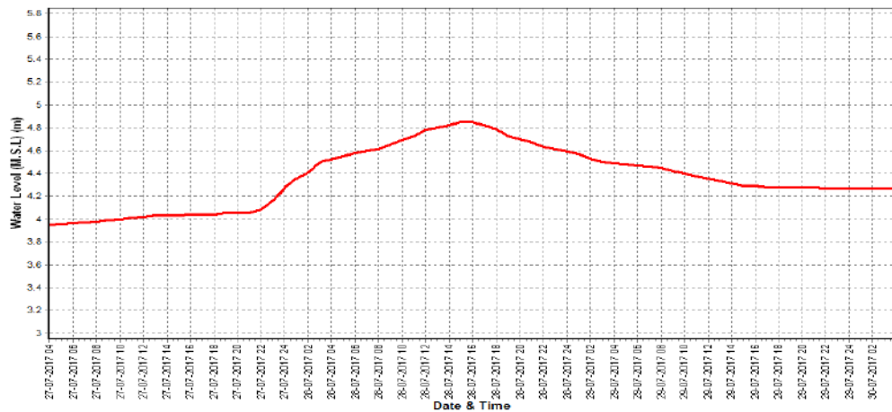
Water Level v/s Time graph of Highest (II) Flood Peak during the water year 2017-18
