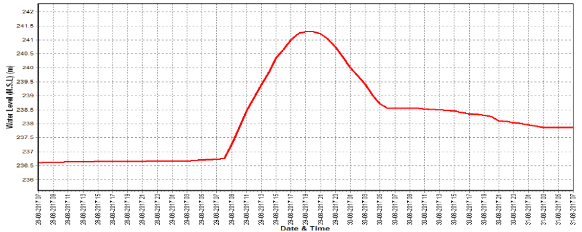
Water level vs Time Graph of Highest (II) flood peak during the water year 2017-18
