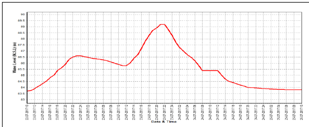
Water level vs. Time graph of I flood peak during the year 2017-18
