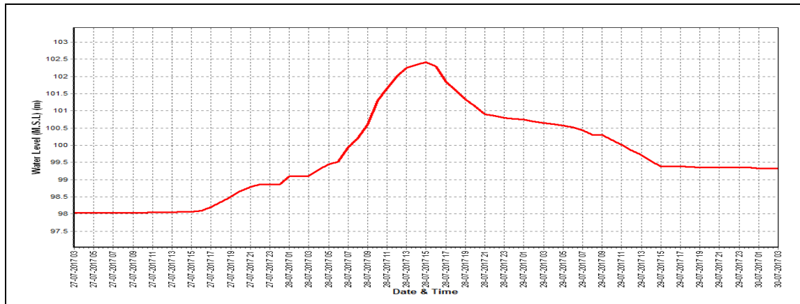
Water level vs. Time graph of II flood peak during the year 2017-18
