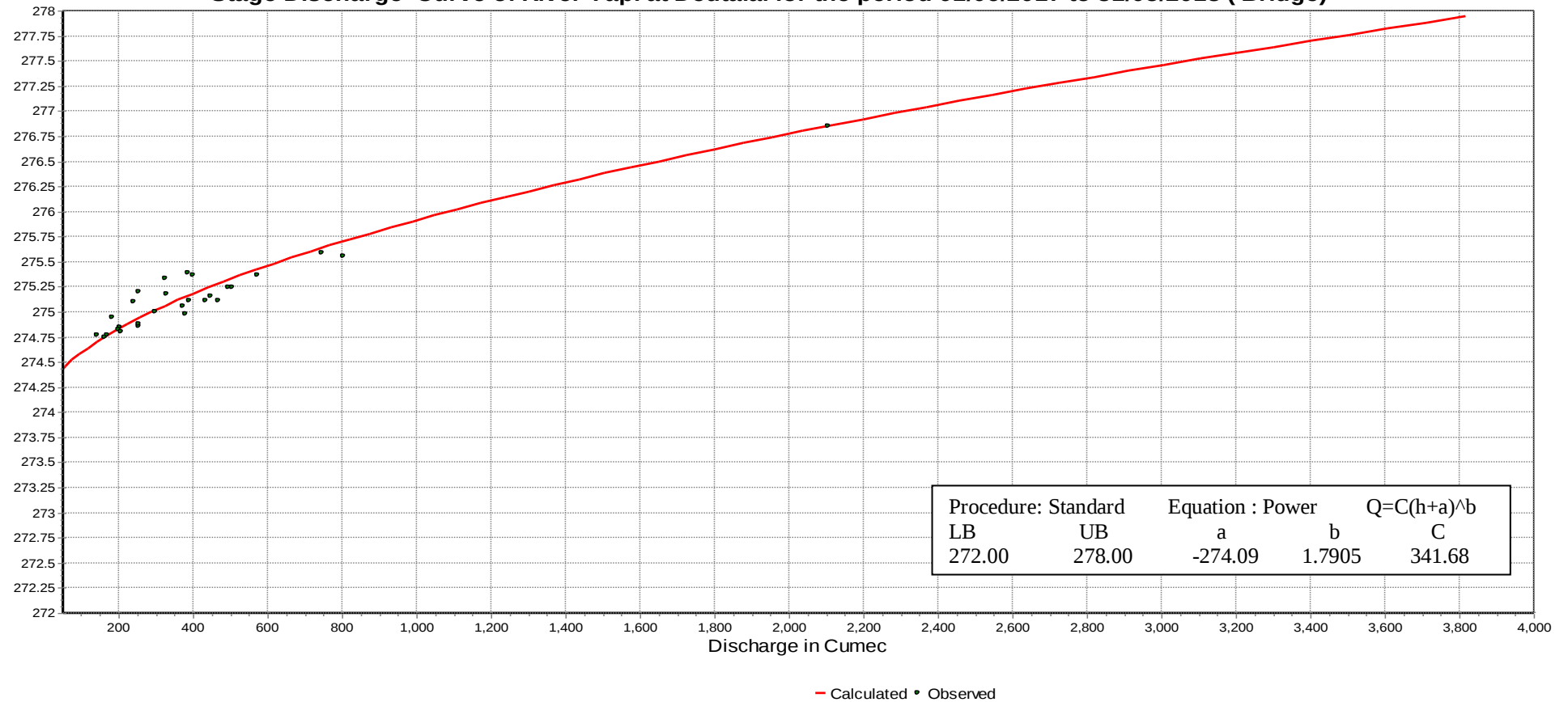
Stage Discharge Curve of River Tapi at Dedtalai for the period 01/06/2017 to 31/05/2018 ( Bridge)
