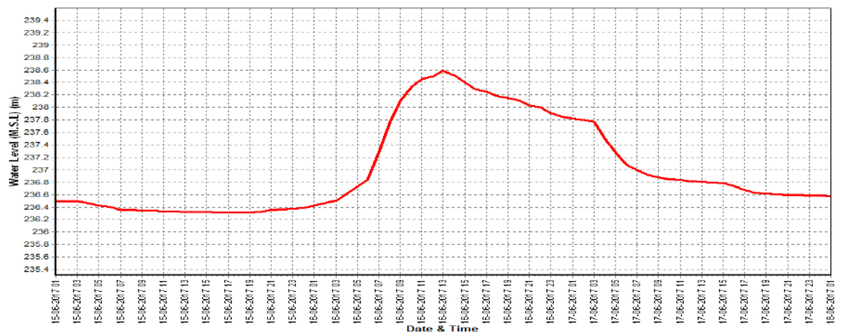
Water level vs Time Graph of Highest (III) flood peak during the water year 2017-18
