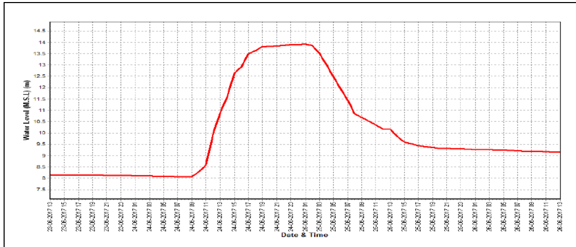
Water level vs. Time graph of 2 nd flood peak during the year 2017-18
