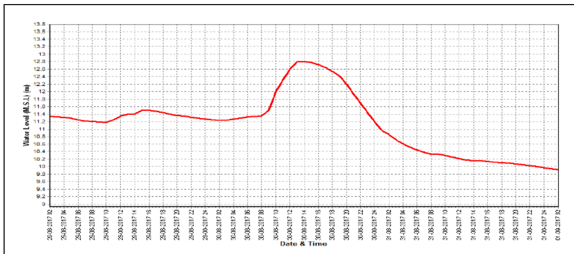
Water level vs. Time graph of 2 nd flood peak during the year 2017-18
