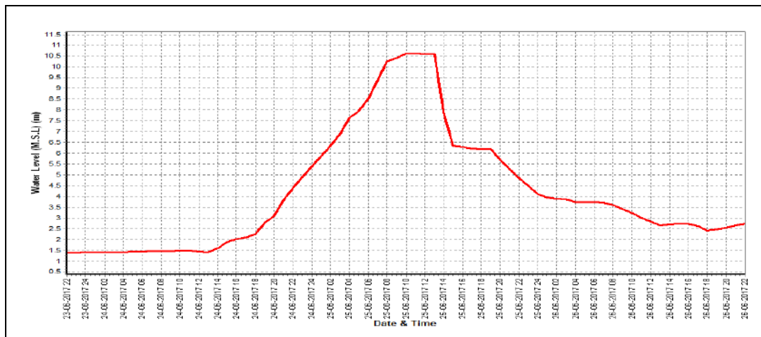
Water level vs. Time graph of II flood peak during the year 2017-18
