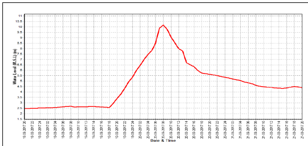
Water level vs. Time graph of III flood peak during the year 2017-18
