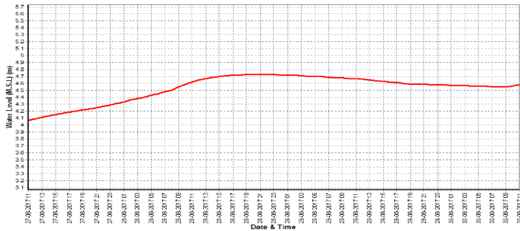
Water Level v/s Time graph of Highest (III) Flood Peak during the water year 2017-18
