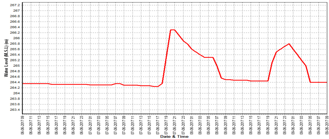
Water level vs Time Graph of Highest (II) flood peak during the water year 2017-18
