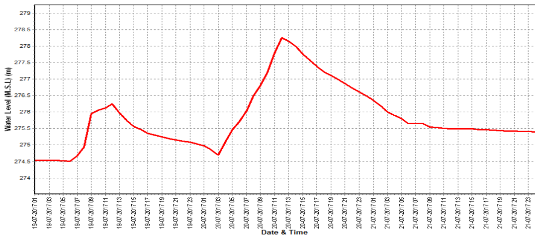
Water Level v/s Time graph of Highest (II) Flood Peak during the water year 2017-18
