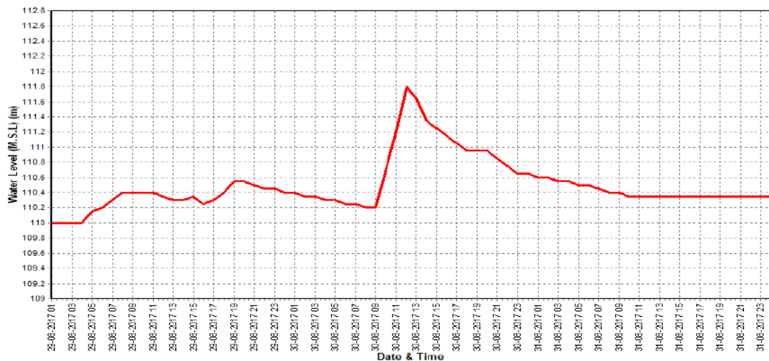
Water Level v/s Time graph of Highest (III) Flood Peak during the water year 2017-18
