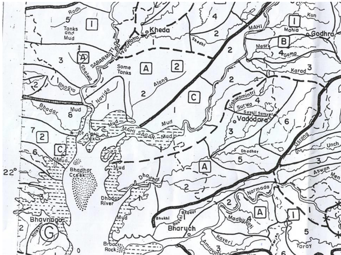
Fig 2.5.1: Sub catchment area of Dhadhar Basin as per water shed Atlas of India.
