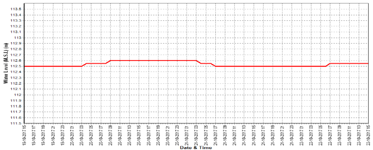
Water Level v/s Time graph of Highest (III) Flood Peak during the water year 2017-18
