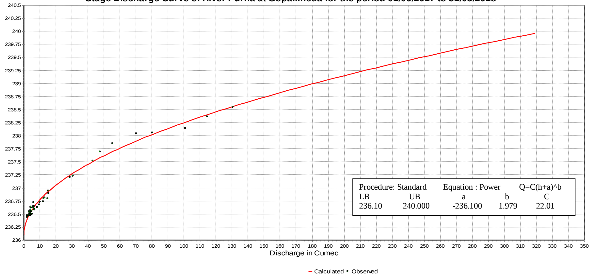
Stage Discharge Curve of River Purna at Gopalkheda for the period 01/06/2017 to 31/05/2018
