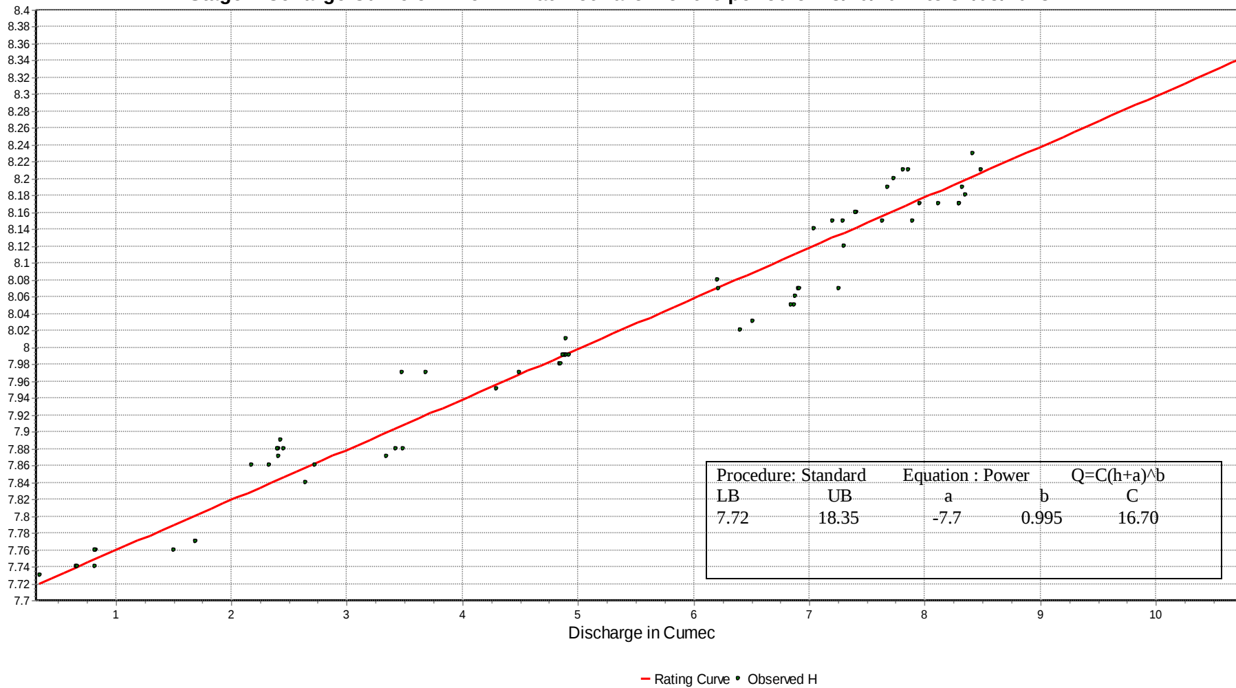
Stage Discharge Curve of River Kim at Motinaroli for the period of 28/10/2017 to 31/05/2018
