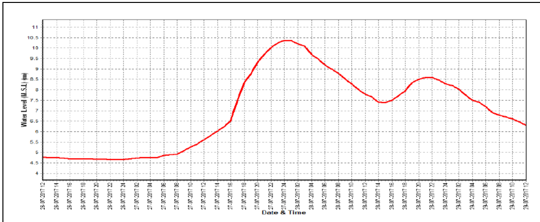
Water level vs. Time graph of 1 st flood peak during the year 2017-18
