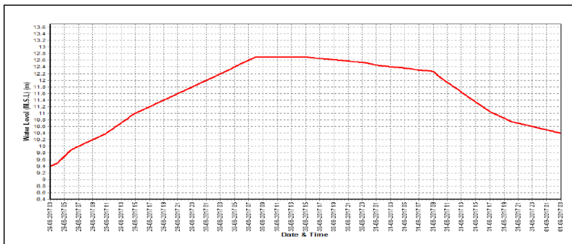
Water level vs. Time graph of II flood peak during the year 2017-18
