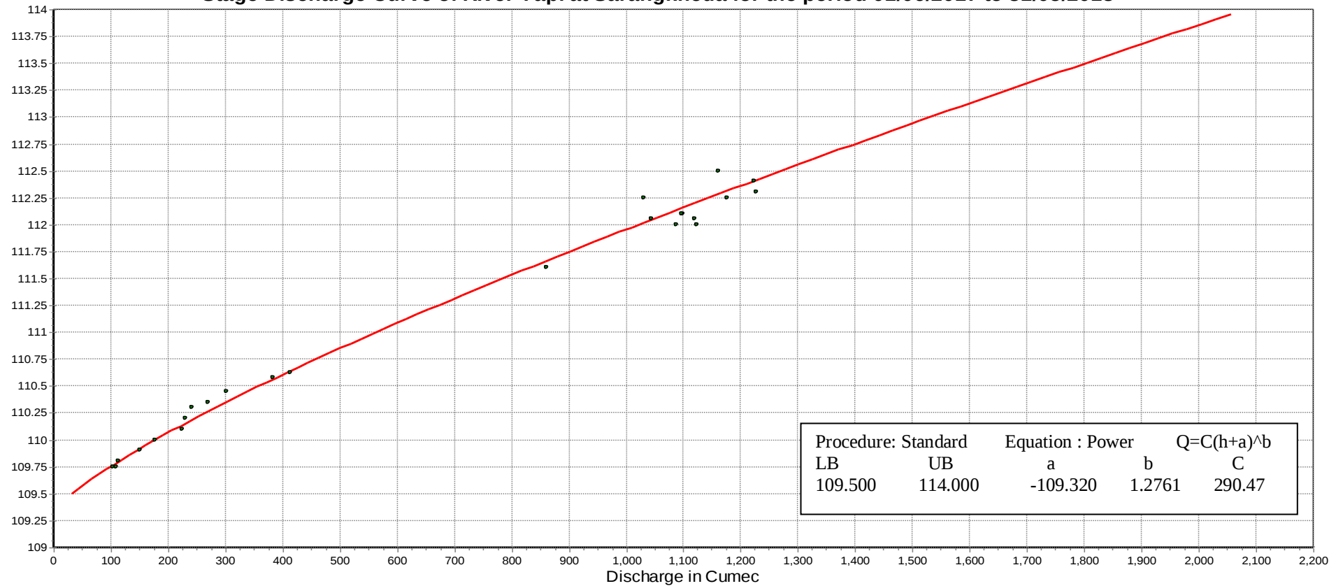
Stage Discharge Curve of River Tapi at Sarangkhedha for the period 01/06/2017 to 31/05/2018
