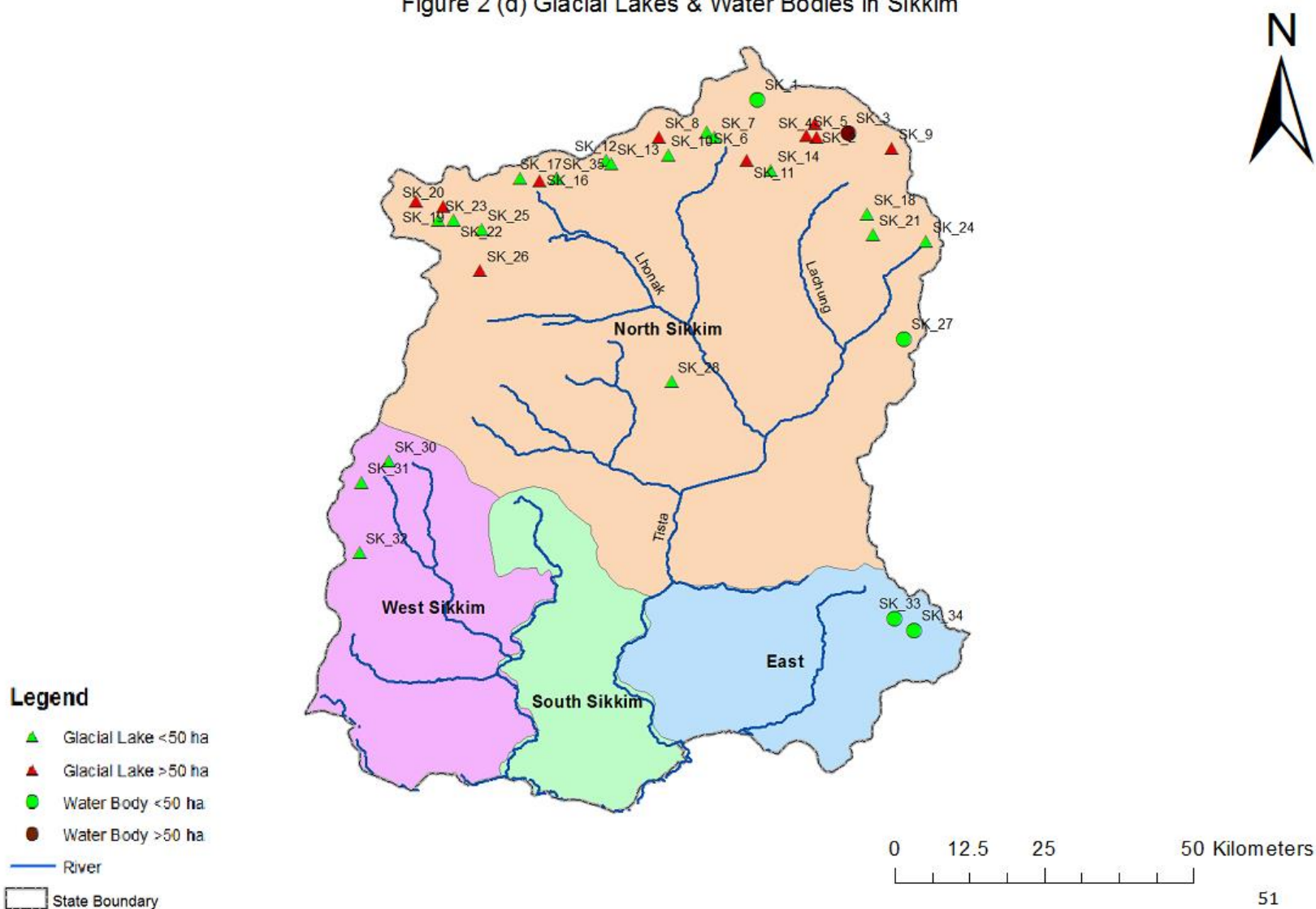
Figure 2 (d) Glacial Lakes & Water Bodies in Sikkim
