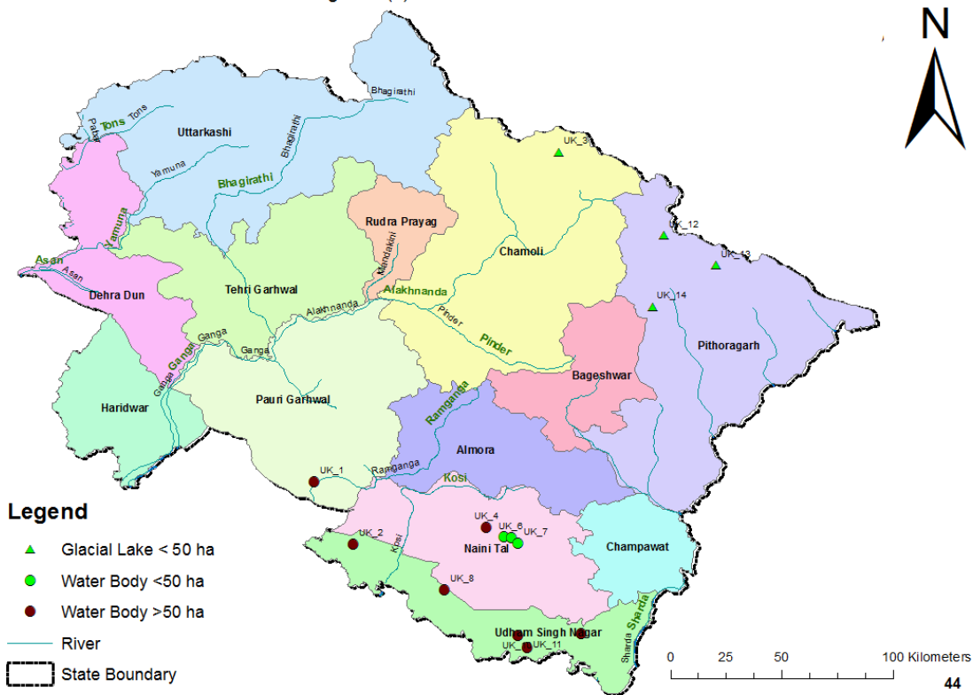
Figure 2 (e) Glacial Lakes & Water Bodies in Uttarakhand
