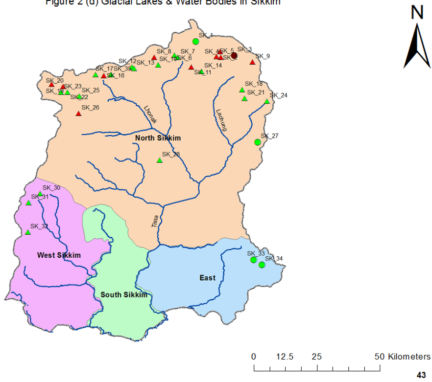
Figure 2 (d) Glacial Lakes & Water Bodies in Sikkim
