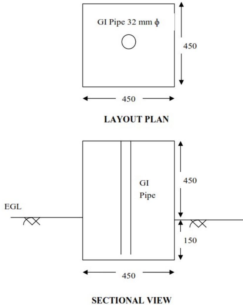
FIG: LAYOUT PLAN AND SECTIONAL VIEW OF PERMANENT BENCHMARK
