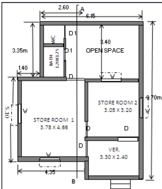
PLAN OF OLD OFFICE BUILDING AT SITE DEROL BRIDGE
