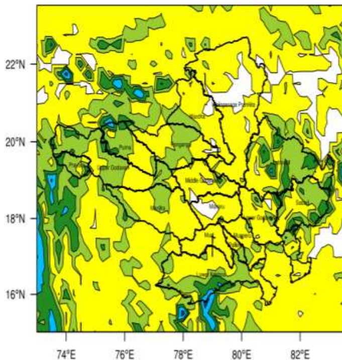
Sub basin wise Average Rainfall Estimation
