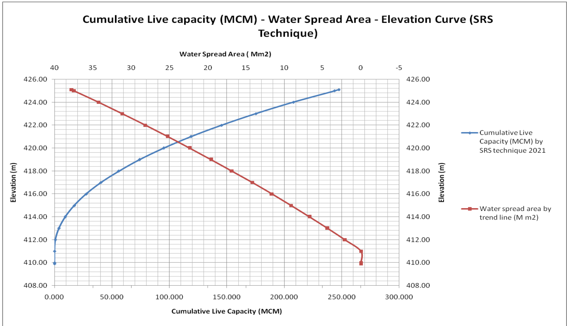
Fig. 10: Elevation – Area- Capacity Curve (Dudhawa Reservoir)
