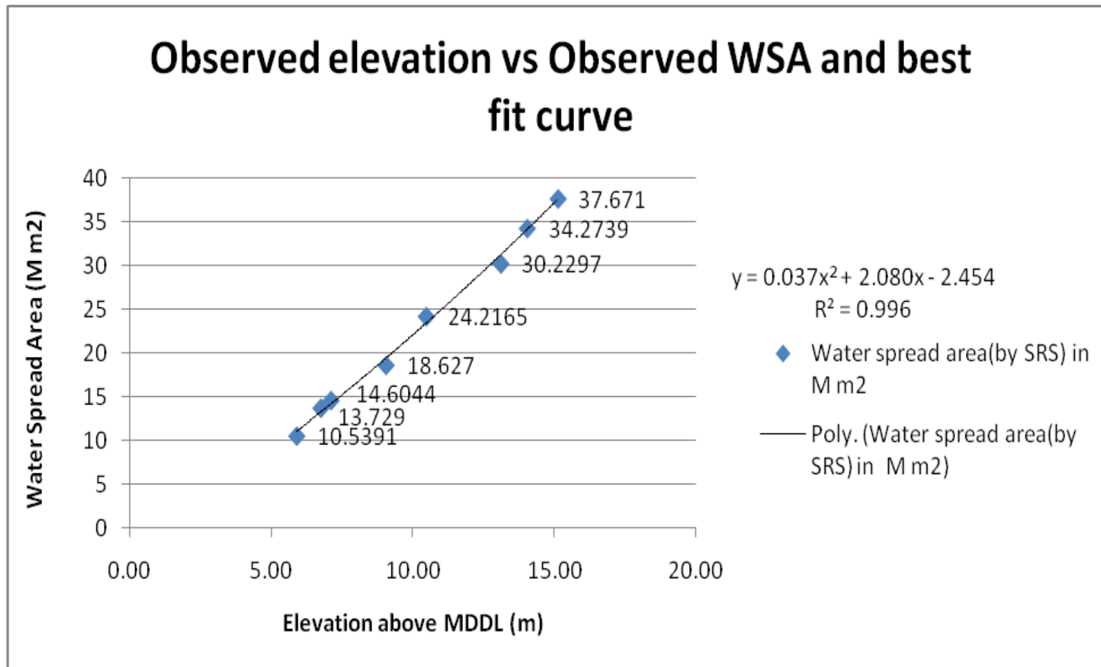
Fig. 8: Observed elevation vs Observed WSA of Dudhawa Reservoir
