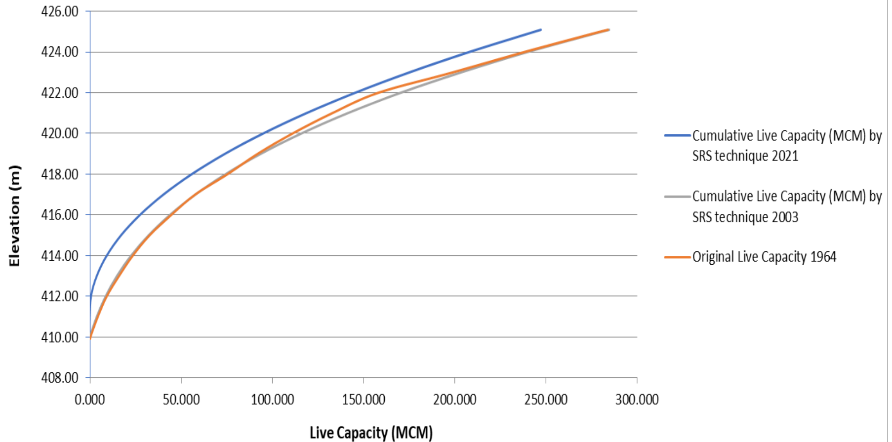
Fig. 11: Comparison of Elevation-Live Storage Capacity Curves (MCM): Dudhawa Reservoir
