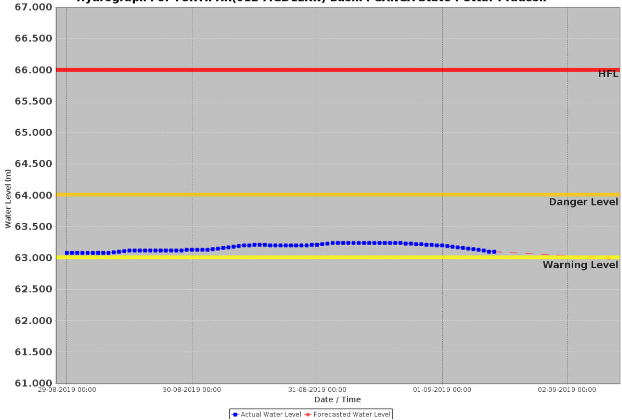
Hydrograph For KACHHLABRIDGE(002-mgd2lkn) Basin : GANGA State : Uttar Pradesh
