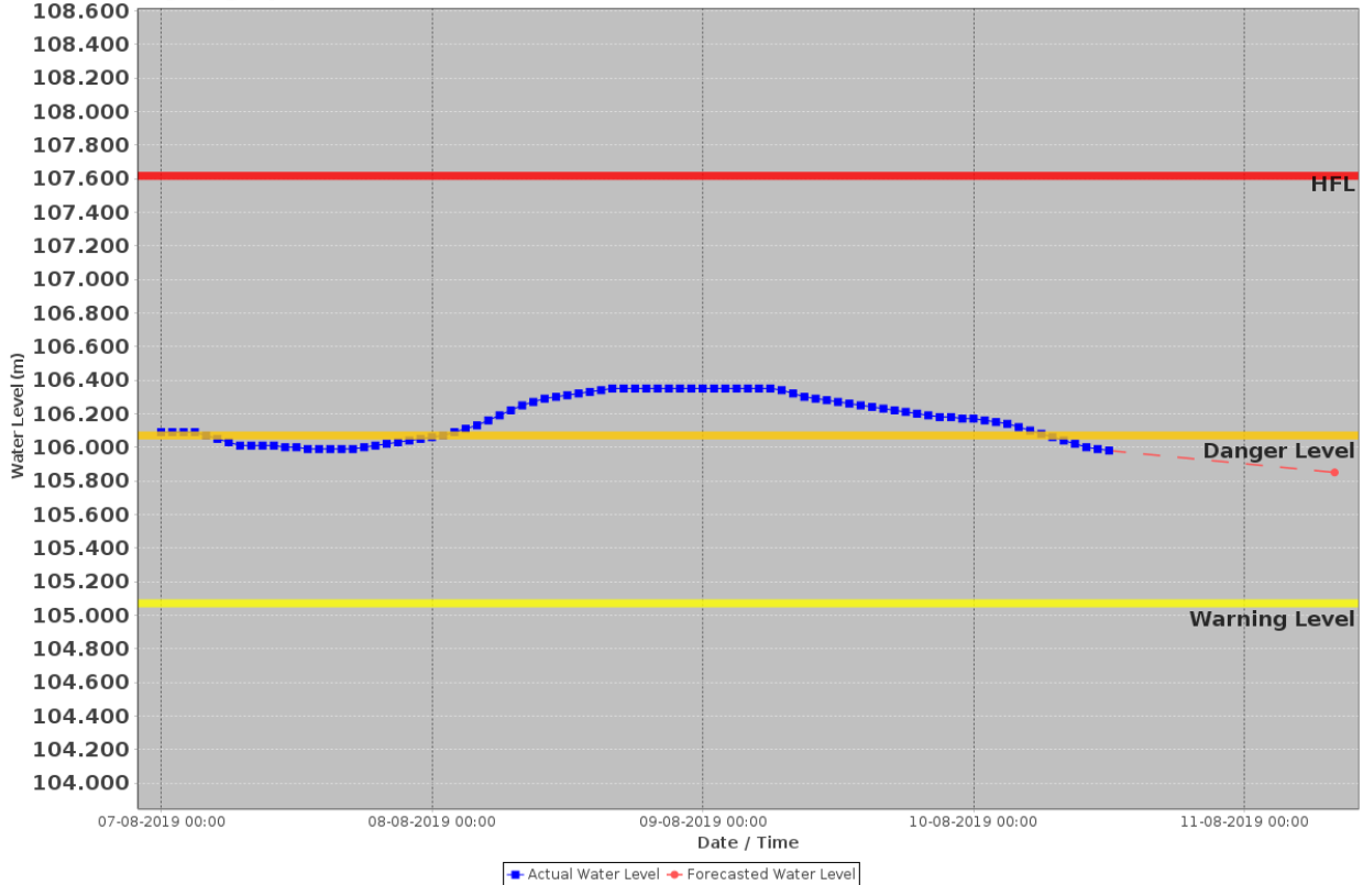
Hydrograph For ELGINBRIDGE(010-MGD1LK) Basin : GANGA State : Uttar Pradesh
