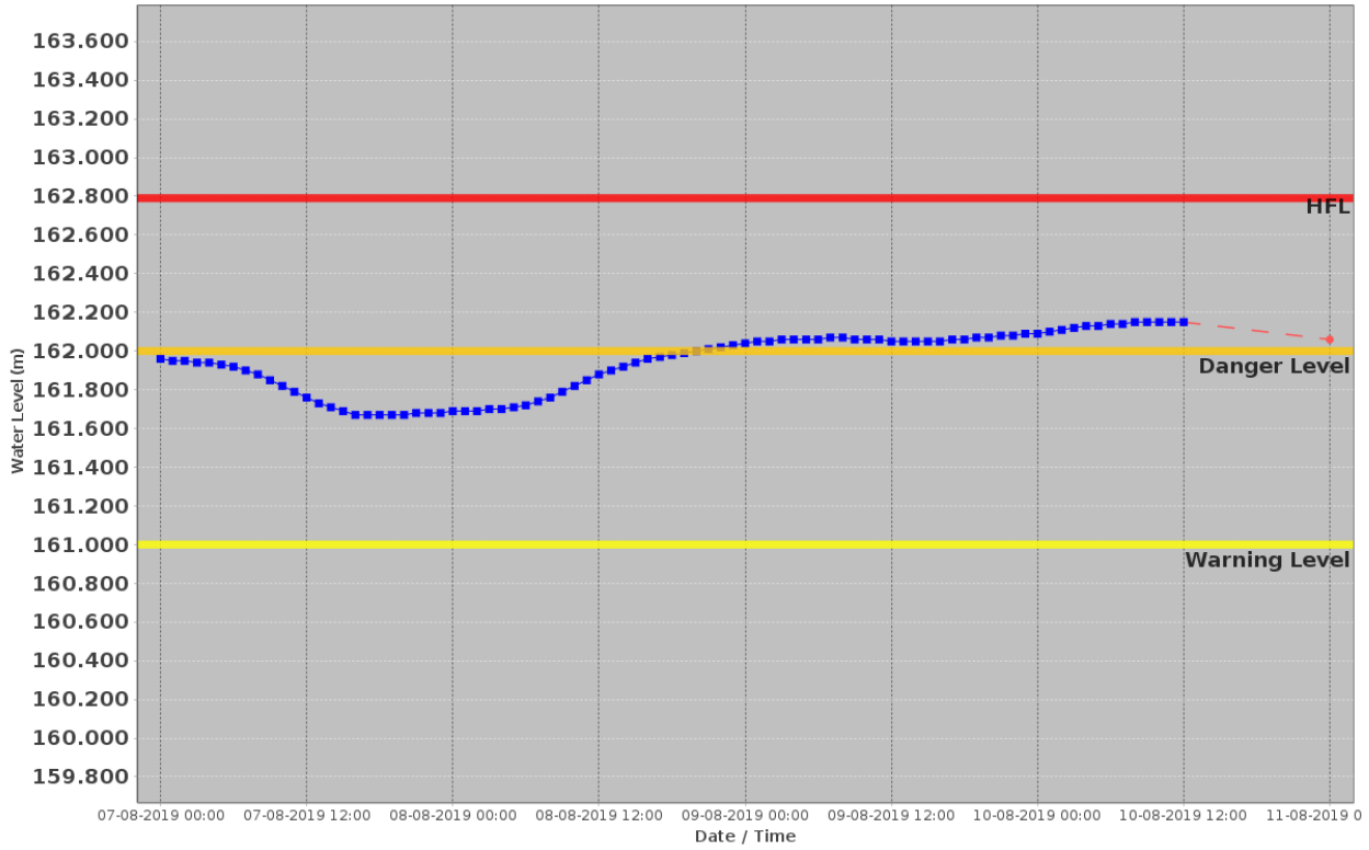
Hydrograph For KACHHLABRIDGE(002-mgd2lkn) Basin : GANGA State : Uttar Pradesh
