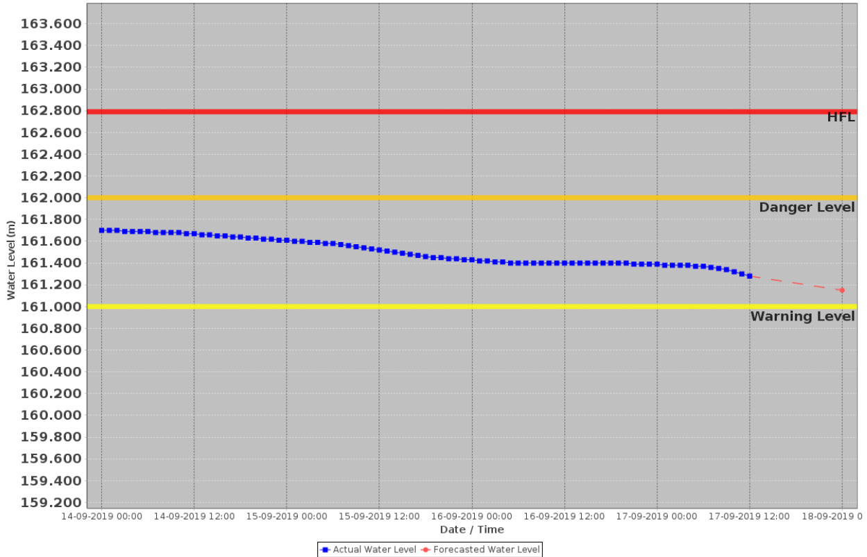
Hydrograph For KACHHLABRIDGE(002-mgd21kn) Basin : GANGA State : Uttar Pradesh
