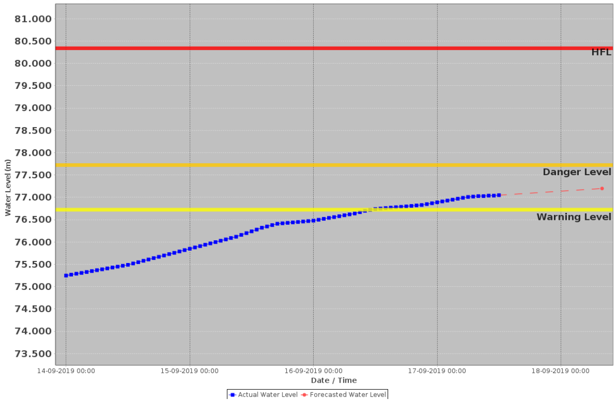
Hydrograph For MIRZAPUR(005-mgd3vns) Basin : GANGA State : Uttar Pradesh
