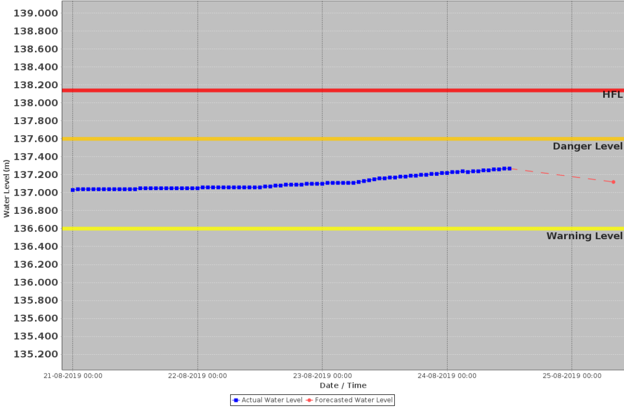
Hydrograph For FATEHGARH(003-mgd21kn) Basin : GANGA State : Uttar Pradesh
