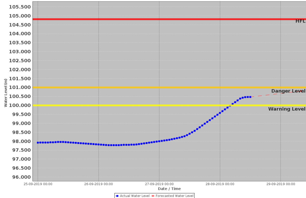
Hydrograph For RAE BARELI(016-mgd21kn) Basin : GANGA State : Uttar Pradesh
