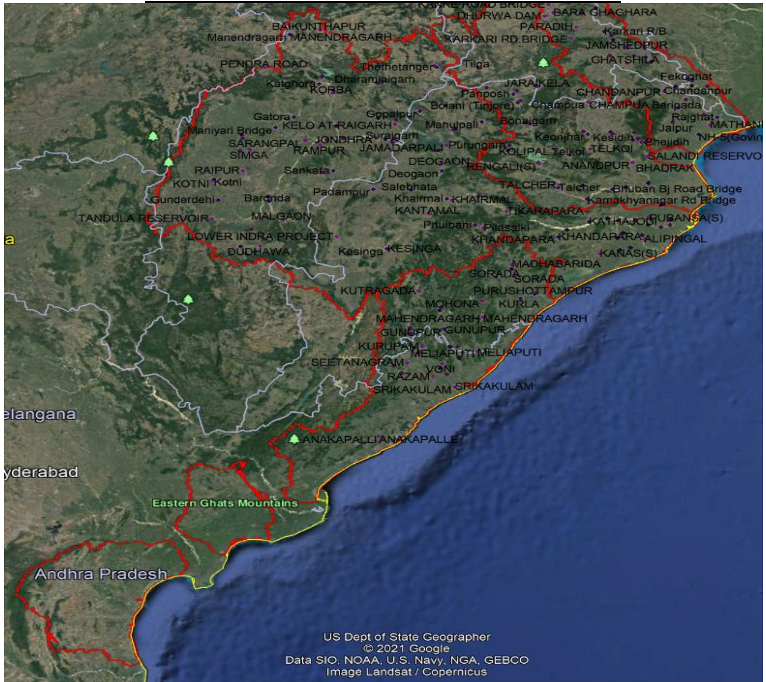
Cloud Cover over sites under M&ERO at 15:00 hours
