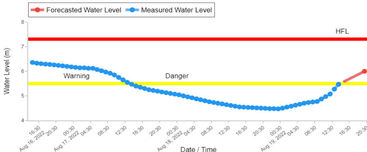
Hydrograph view of - Mathani Road Bridge
