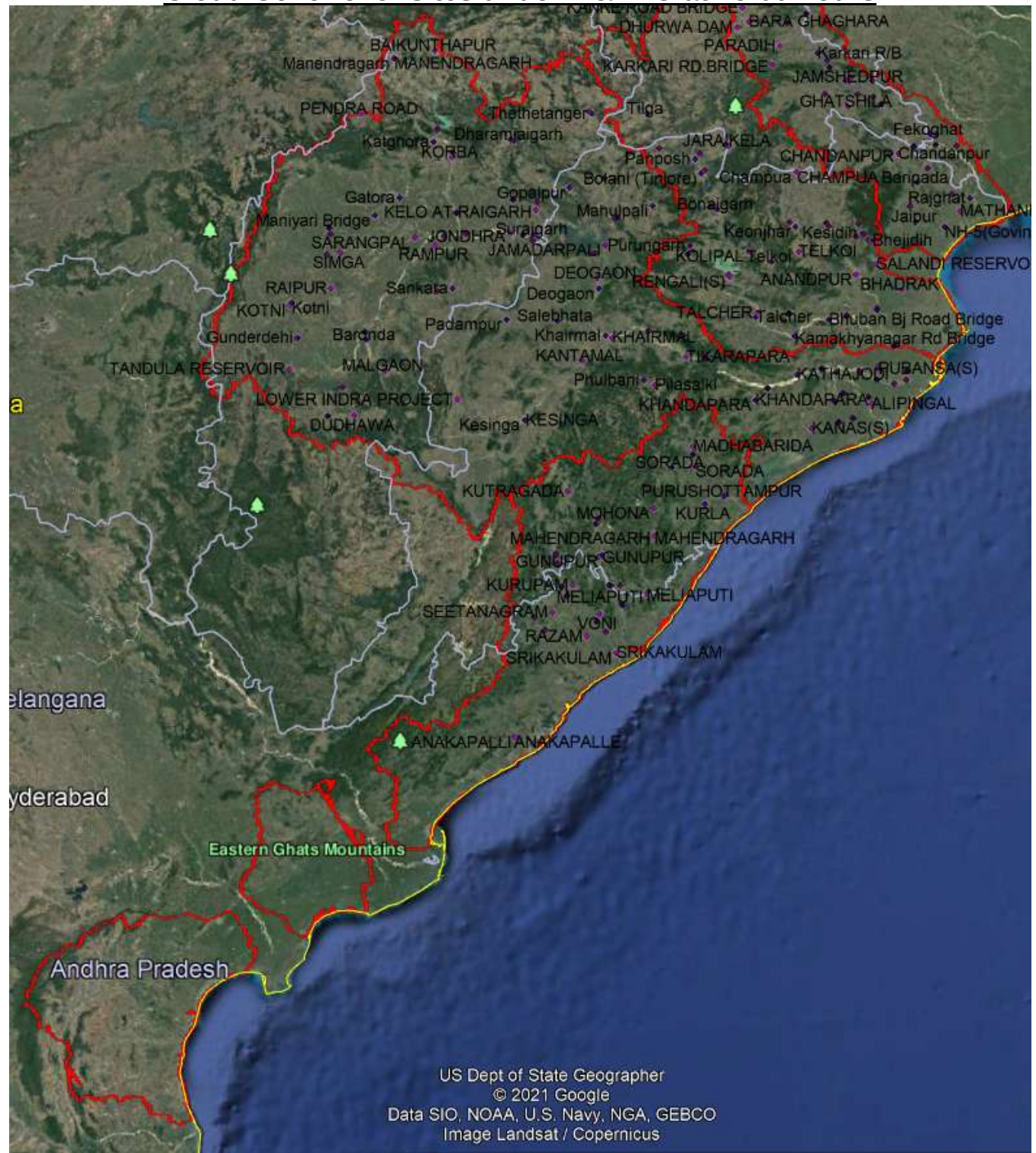
Cloud Cover over sites under M&ERO at 15:00 hours
