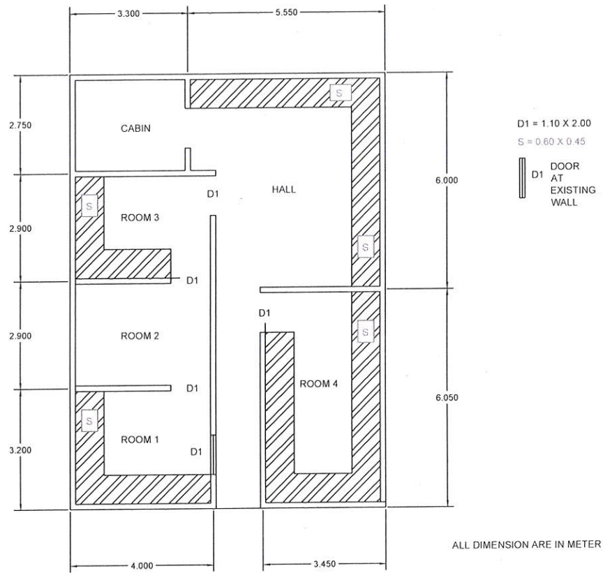
PLAN OF LEVEL II LABORATORY AT SWRD, KOCHI
