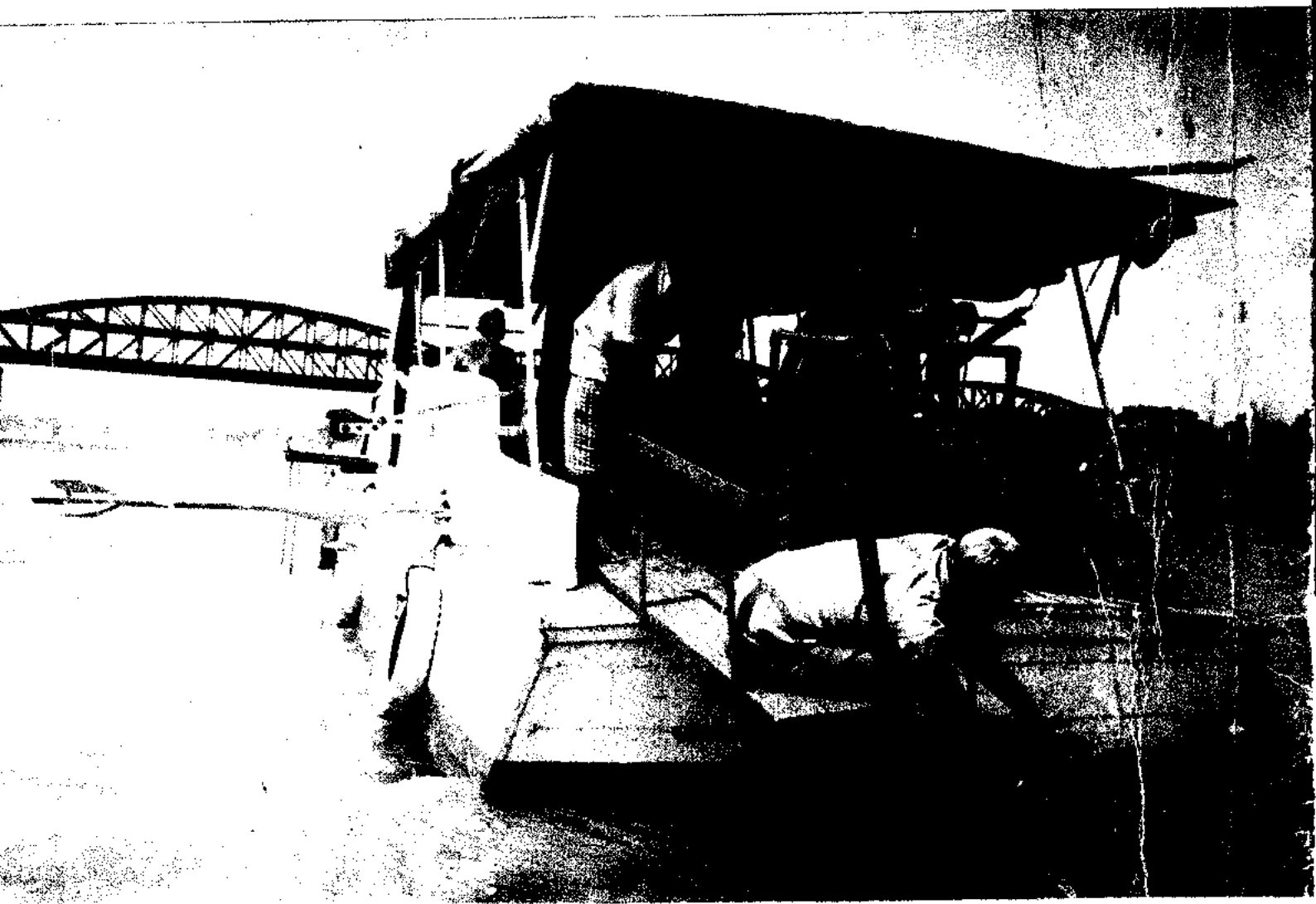
Discharge Observation In Ganga At Varanasi
