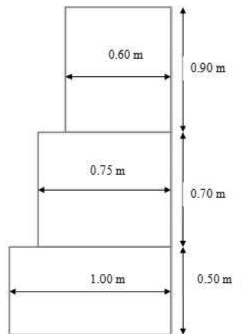
Elevation of Retaining Wall
