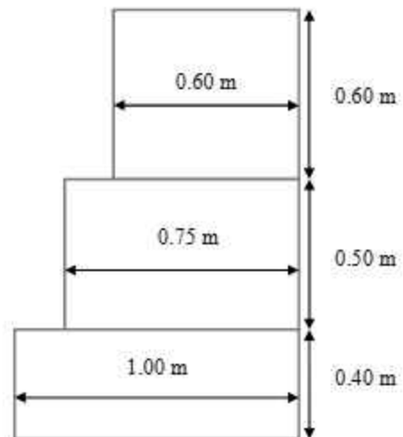
Elevation of Retaining Wall
