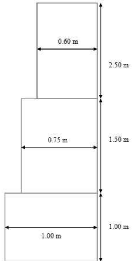
Elevation of Retaining Wall
