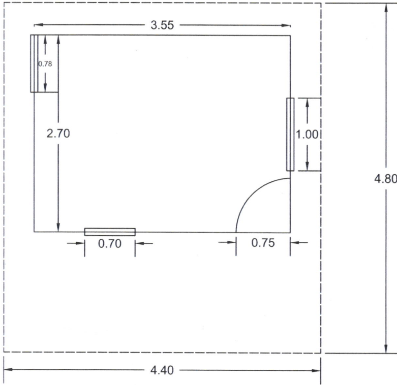
Plane View
