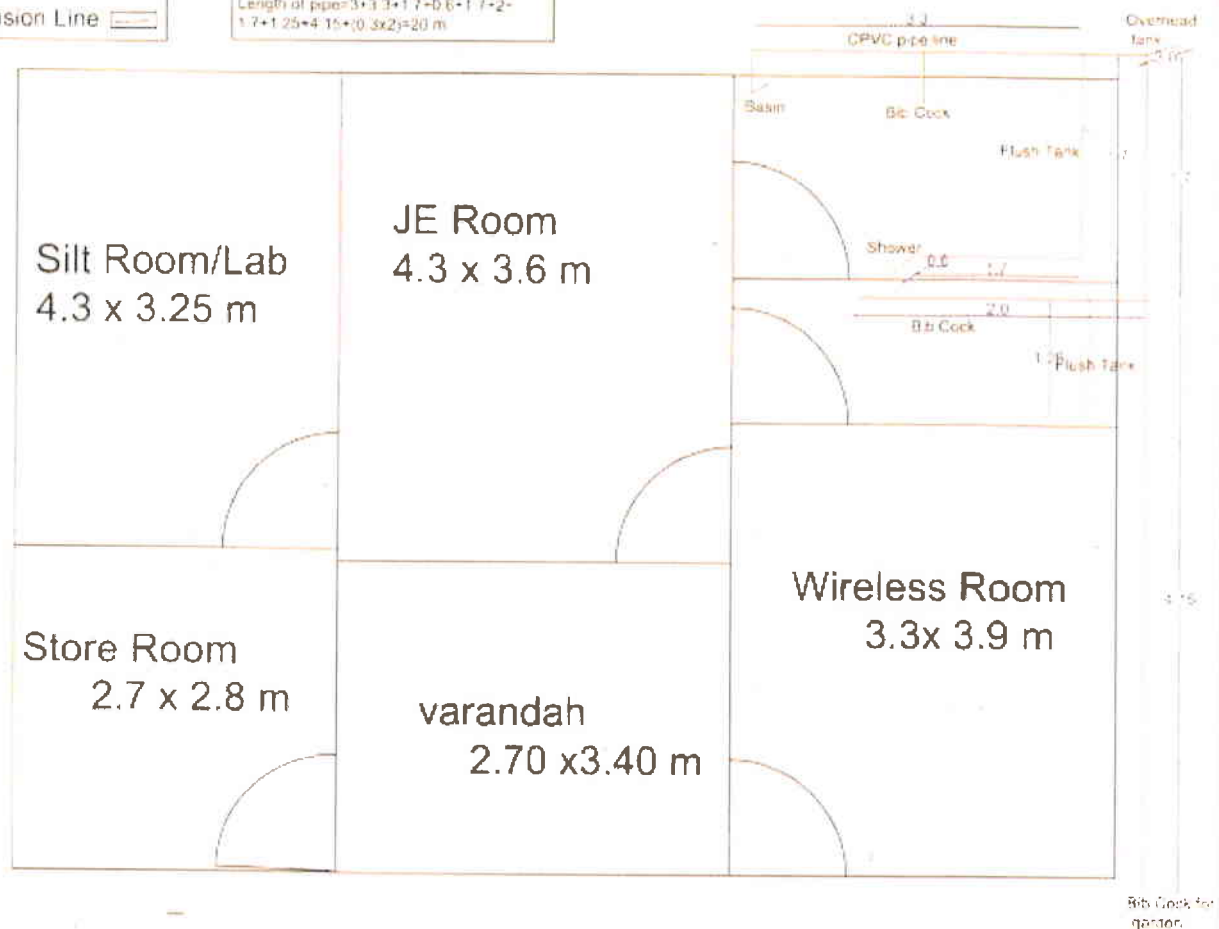
Building outline and Plumbing plan at Site Office Building Nandgaon under PGSD Yavatmal
