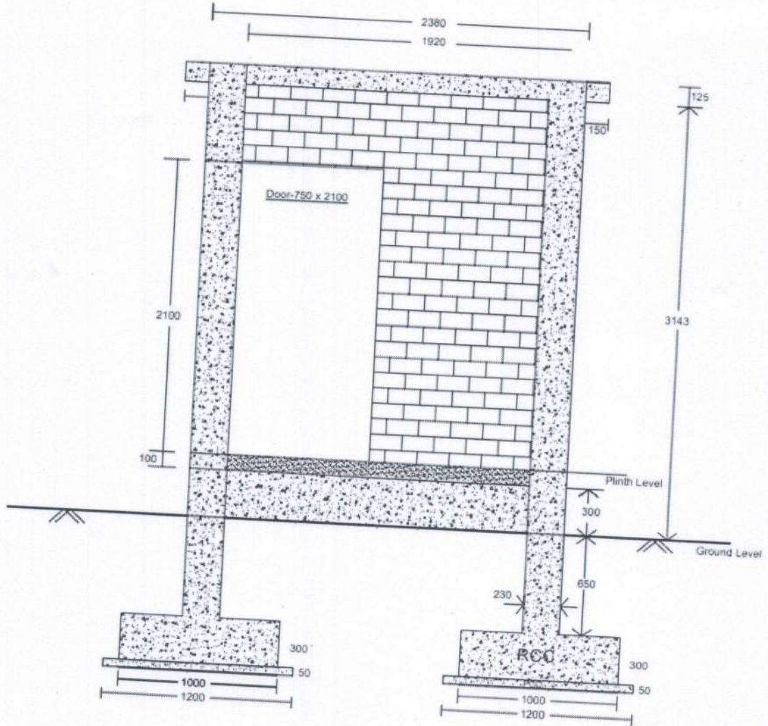
Front Sectional Elevation
