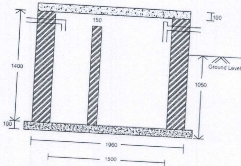
Septic Tank Elevation
