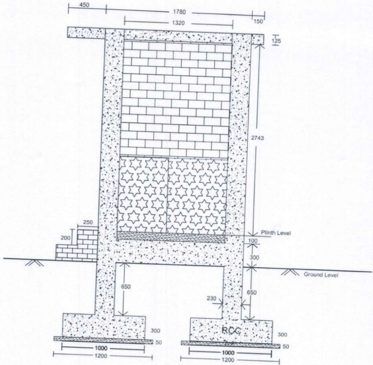
Side Sectional Elevation
