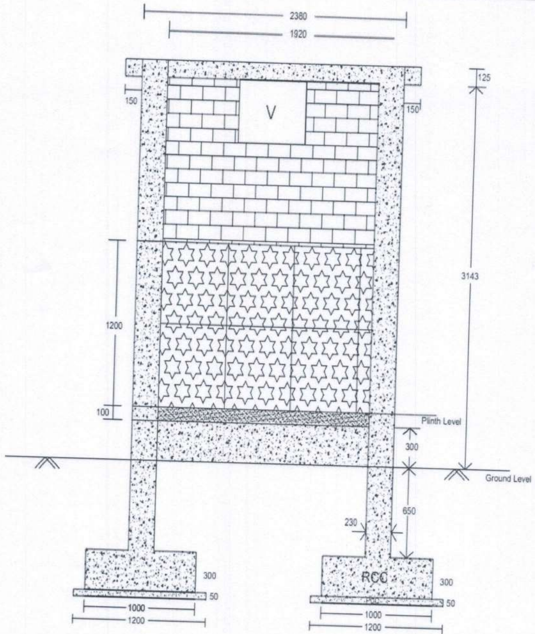
Section Elevation at AA'
