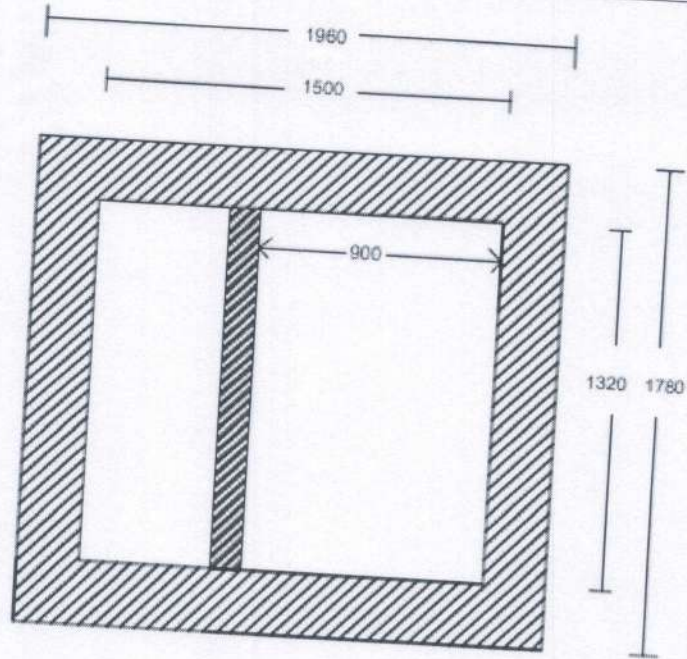
Septic Tank Plan
