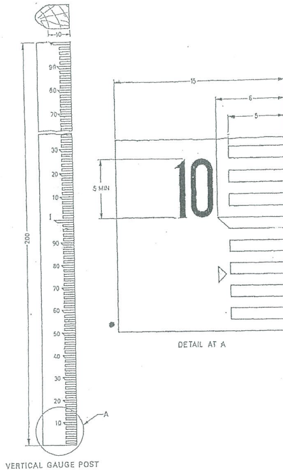
FIG. 1 TYPICAL DETAILS OF VERTICAL STAFF GAUGE
