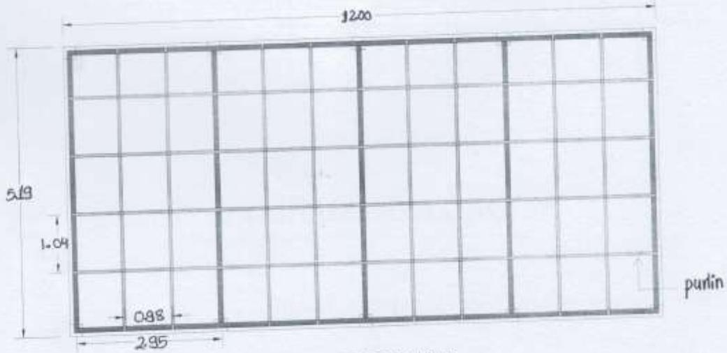
ROOF FRAME DETAILS
