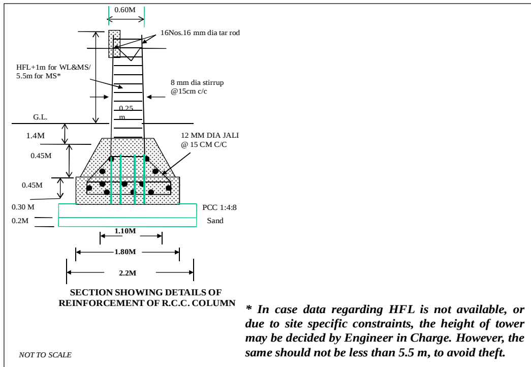
Drawing 2: Layout of Concrete Pillar - details
