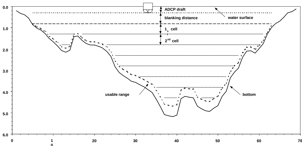
Figure 6.45(d): Effects of depth, draft and blanking on profile
