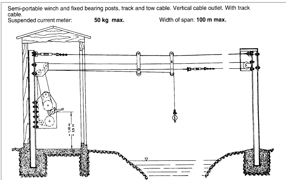
Figure 6.28: Unmanned Cableway System
