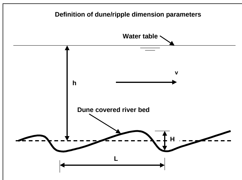
Figure 2.3: Dune/ripple dimension parameters
