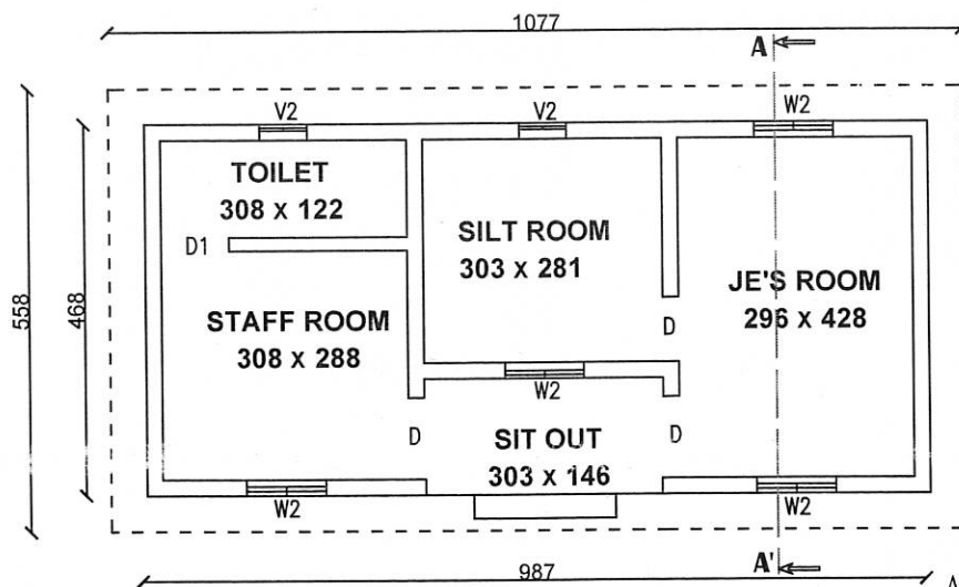
PLAN OF SITE OFFICE THUMPAMON (SP SHED)
