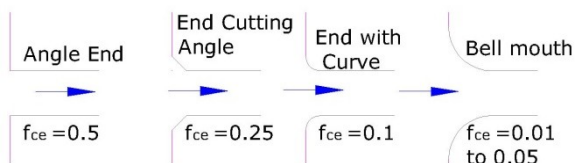
Figure 3.5 Shape of Inlet and Loss Coefficient
