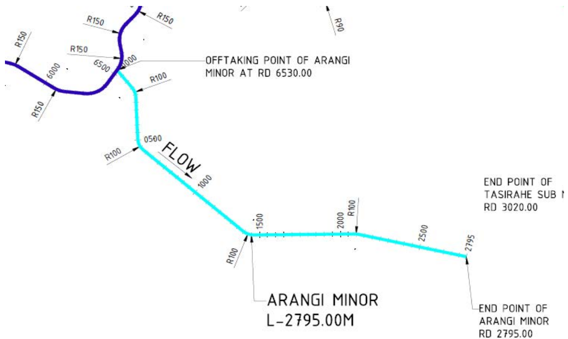
Figure 10.3 Alignment of Arangi Minor with RD and curves
