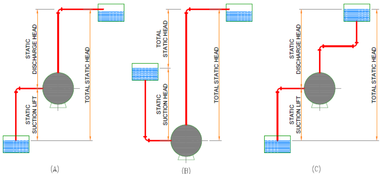
Figure 7.1 Head terms used in Pumping
