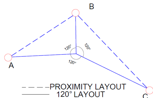
Figure 5.8 120^\circ Layout - Case of 3 Hydrants
