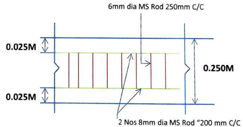
Plan View at Ground Level.
