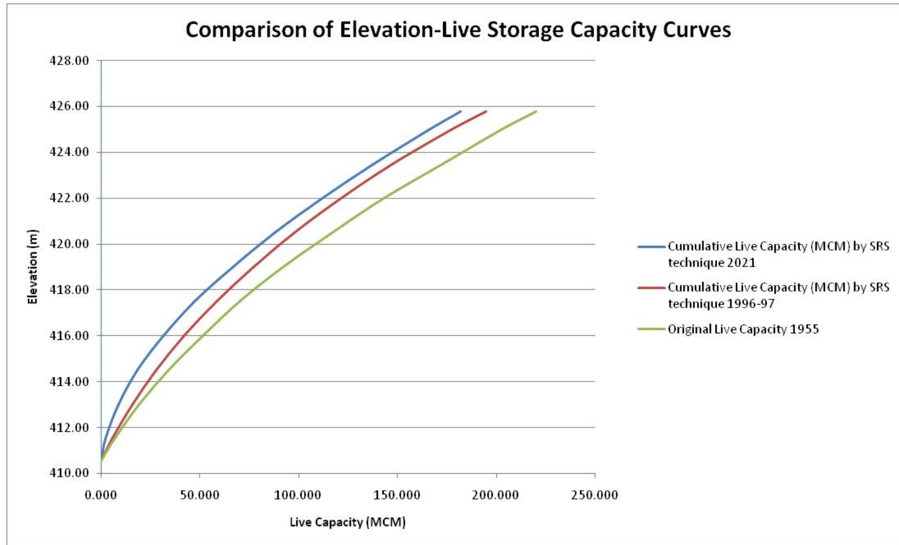
Fig. 11: Comparison of Elevation-Live Storage Capacity Curves (MCM): Konar Reservoir
