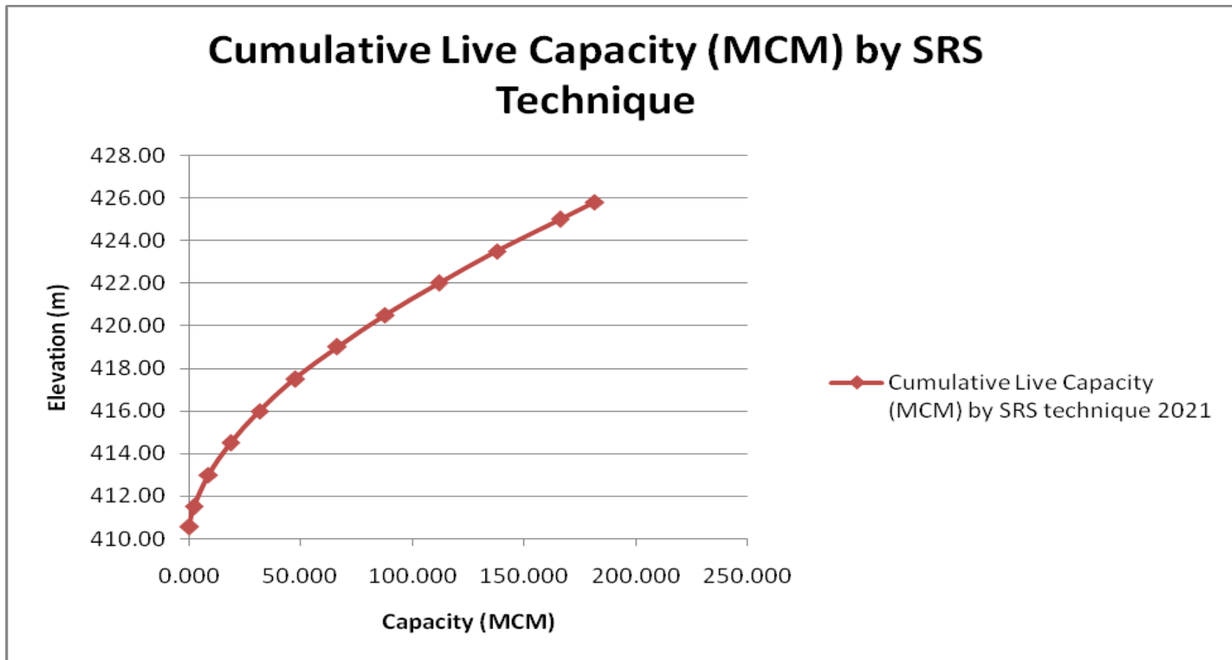
Fig. 9: Modified live capacity - elevation curve (SRS technique) : Konar Reservoir
