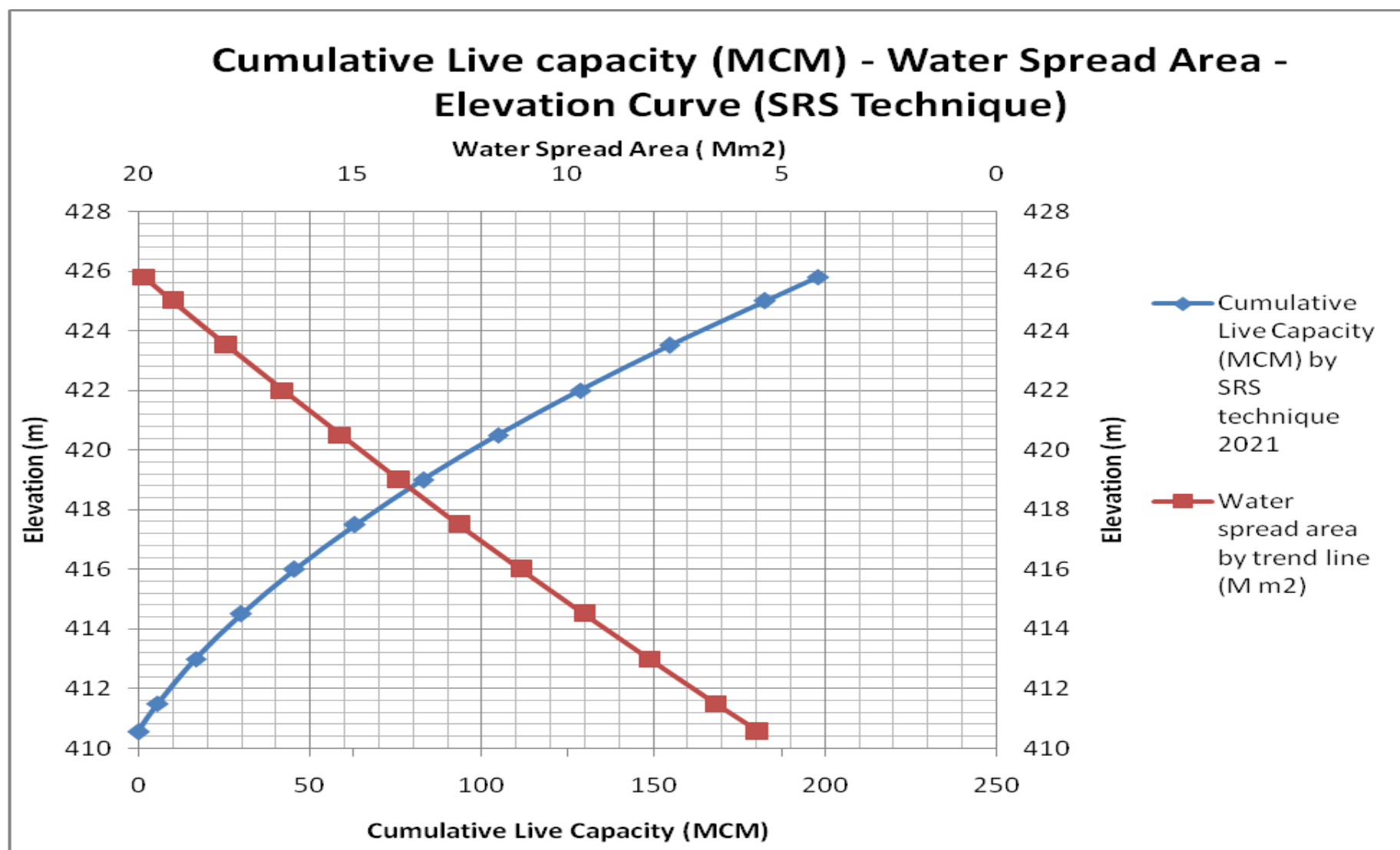
Fig. 10: Elevation – Area- Capacity Curve (Konar Reservoir)
