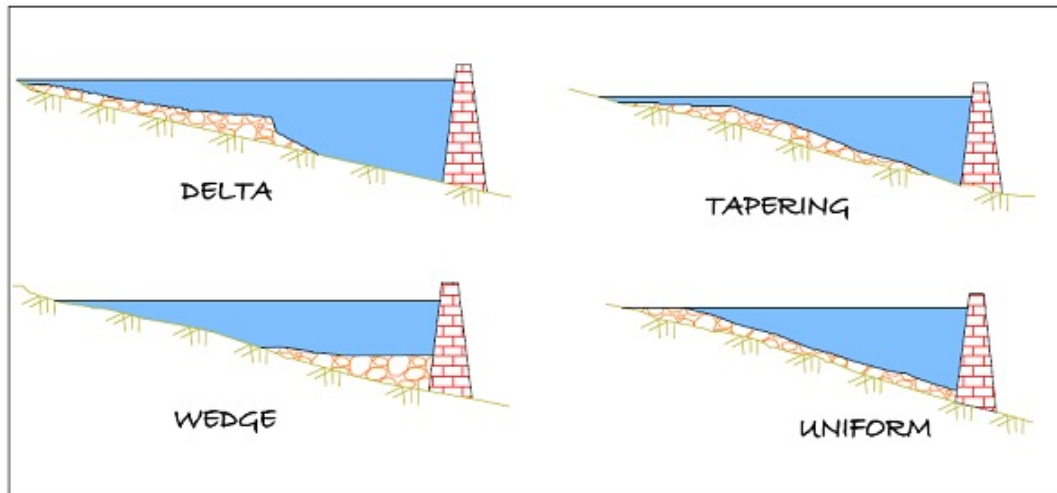
Figure 2: Longitudinal Patterns of sediment deposition in reservoirs
