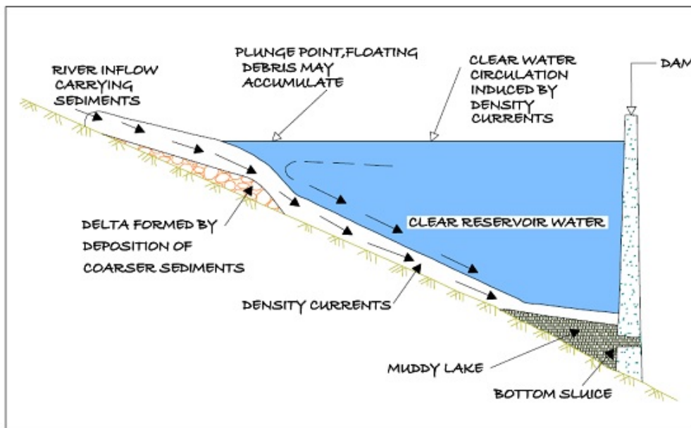
Figure 1: Conceptual sketch of density currents in a reservoir
