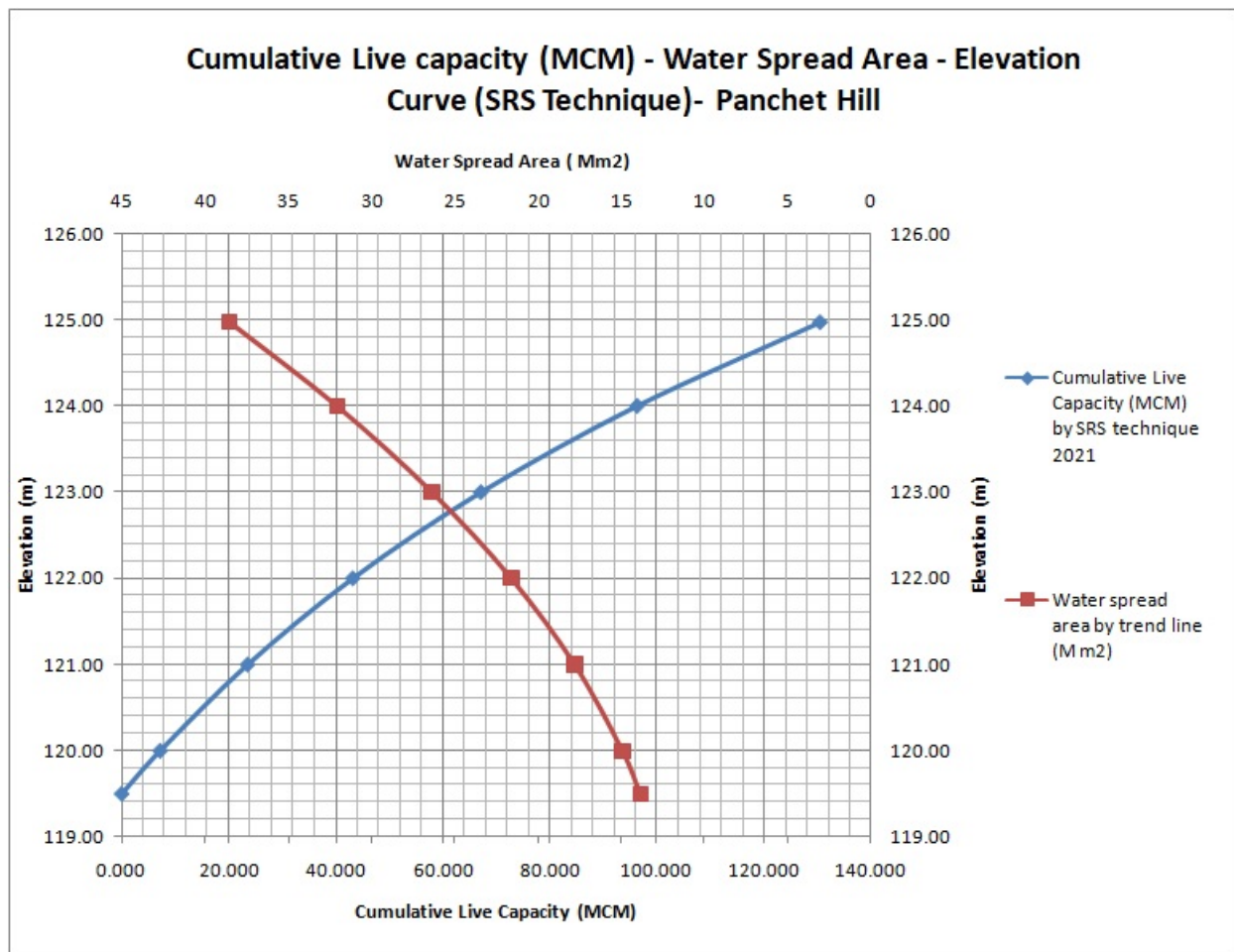
Figure 9: Elevation – Area- Capacity Curve (Panchet Reservoir)
