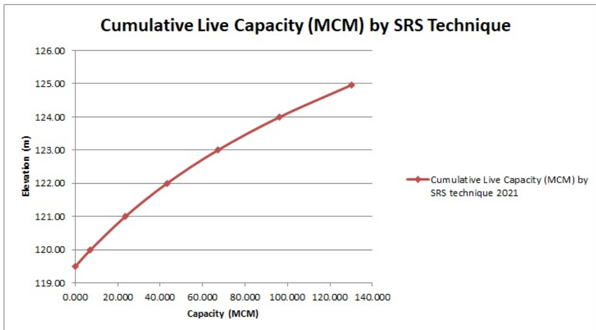
Figure 8: Modified live capacity - elevation curve (SRS technique) : Panchet Reservoir
