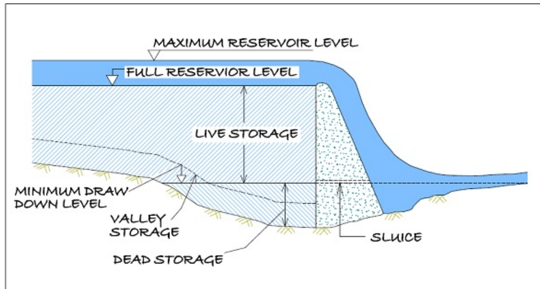
Figure 3: Conceptual sketch of different levels in a reservoir
