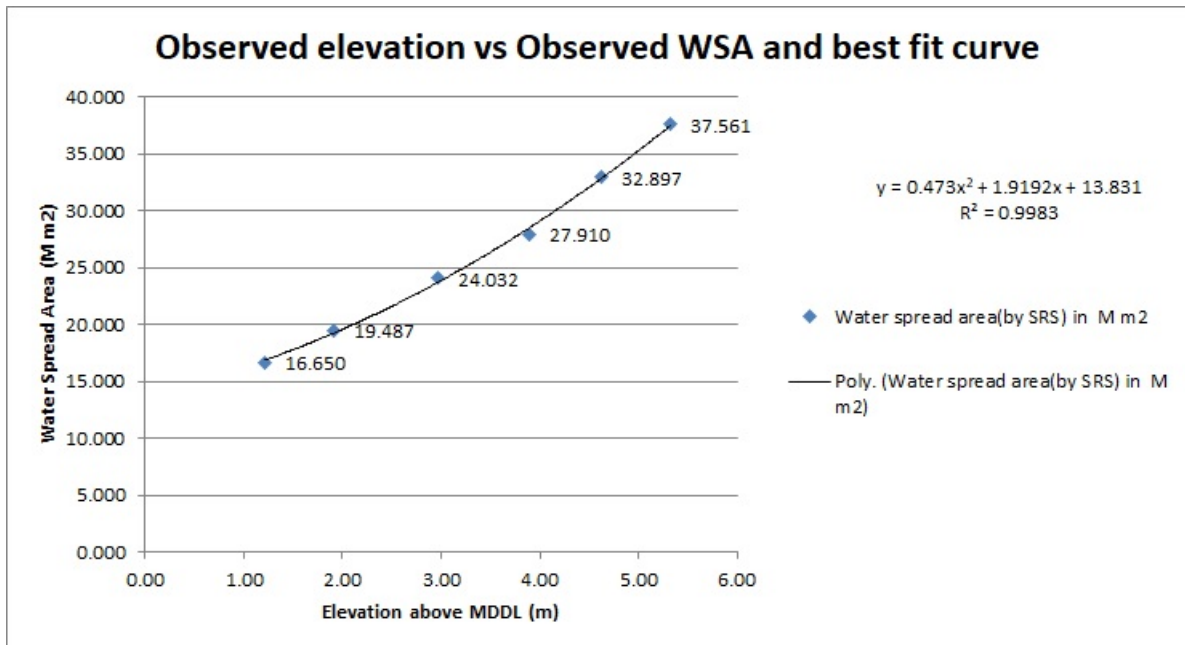
Figure 7: Observed elevation vs Observed WSA of Panchet Reservoir
