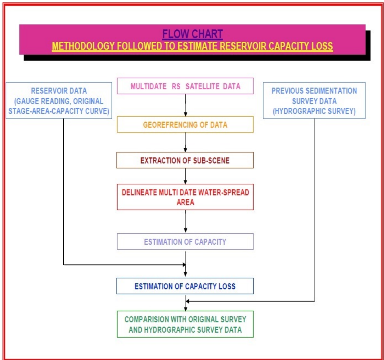
Figure 5: Flow chart showing methodology followed to estimate reservoir capacity loss
