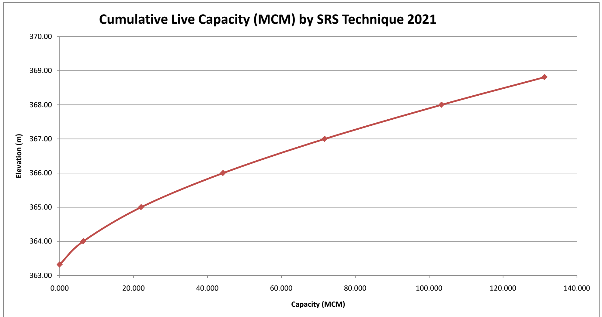
Fig. 9: Modified live capacity - elevation curve (SRS technique)-Tilaiya reservoir, Jharkhand
