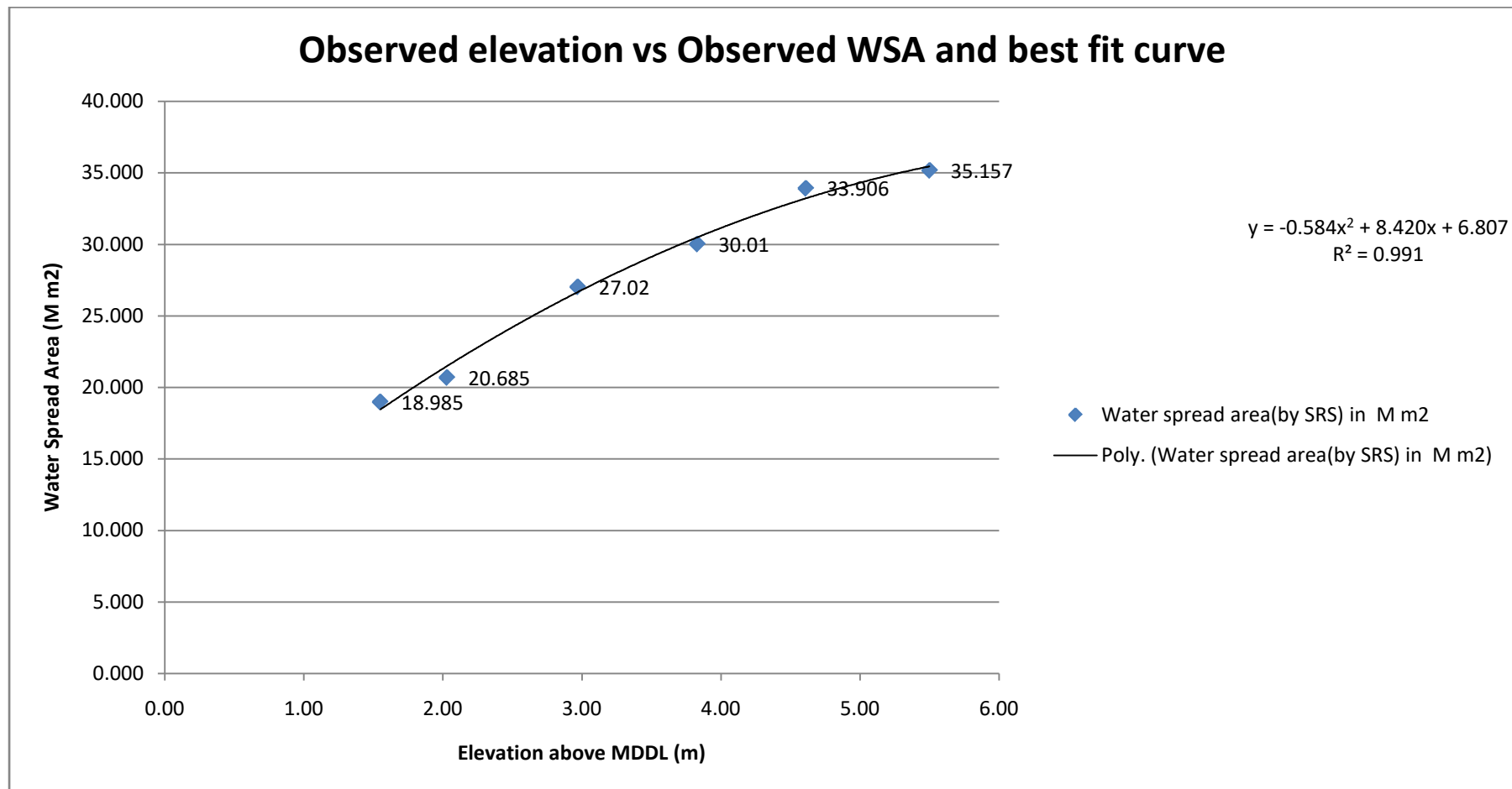
Fig. 8: Observed Elevation vs Observed WSA of Tilaiya reservoir, Jharkhand
