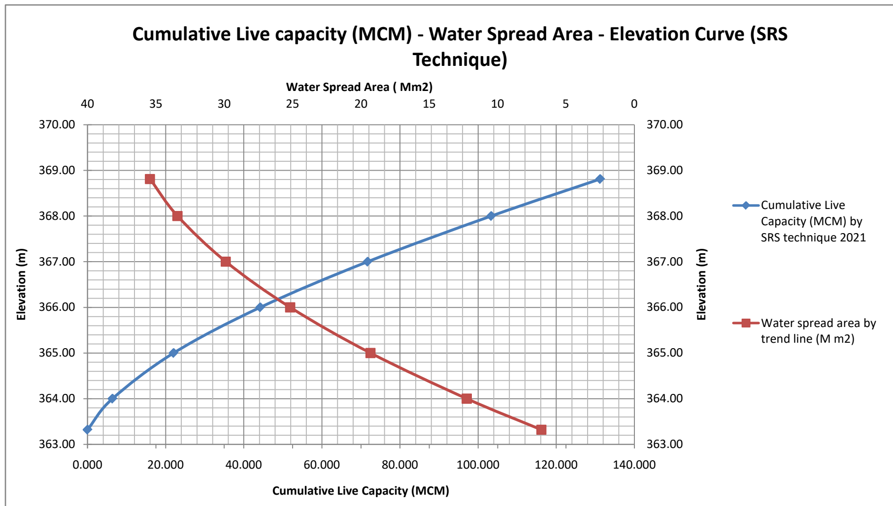
Fig. 10: Elevation – Area- Capacity Curve- Tilaiya reservoir, Jharkhand
