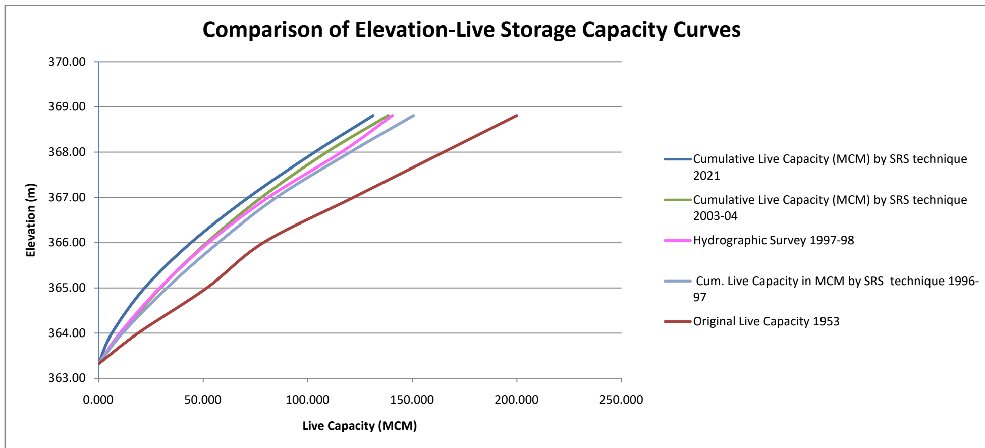
Fig. 11: Comparison of Elevation-Live Storage Capacity Curves (MCM)- Tilaiya reservoir, Jharkhand
