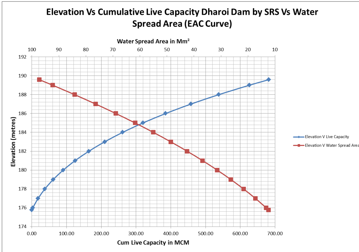
Fig. 10: Elevation – Area – Capacity Curve
