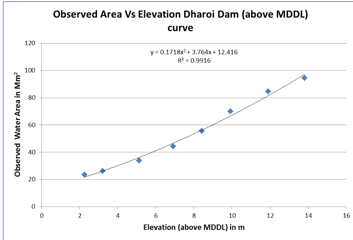
Fig. 8: Observed elevation vs Observed Water Spread Area of Dharoi reservoir
