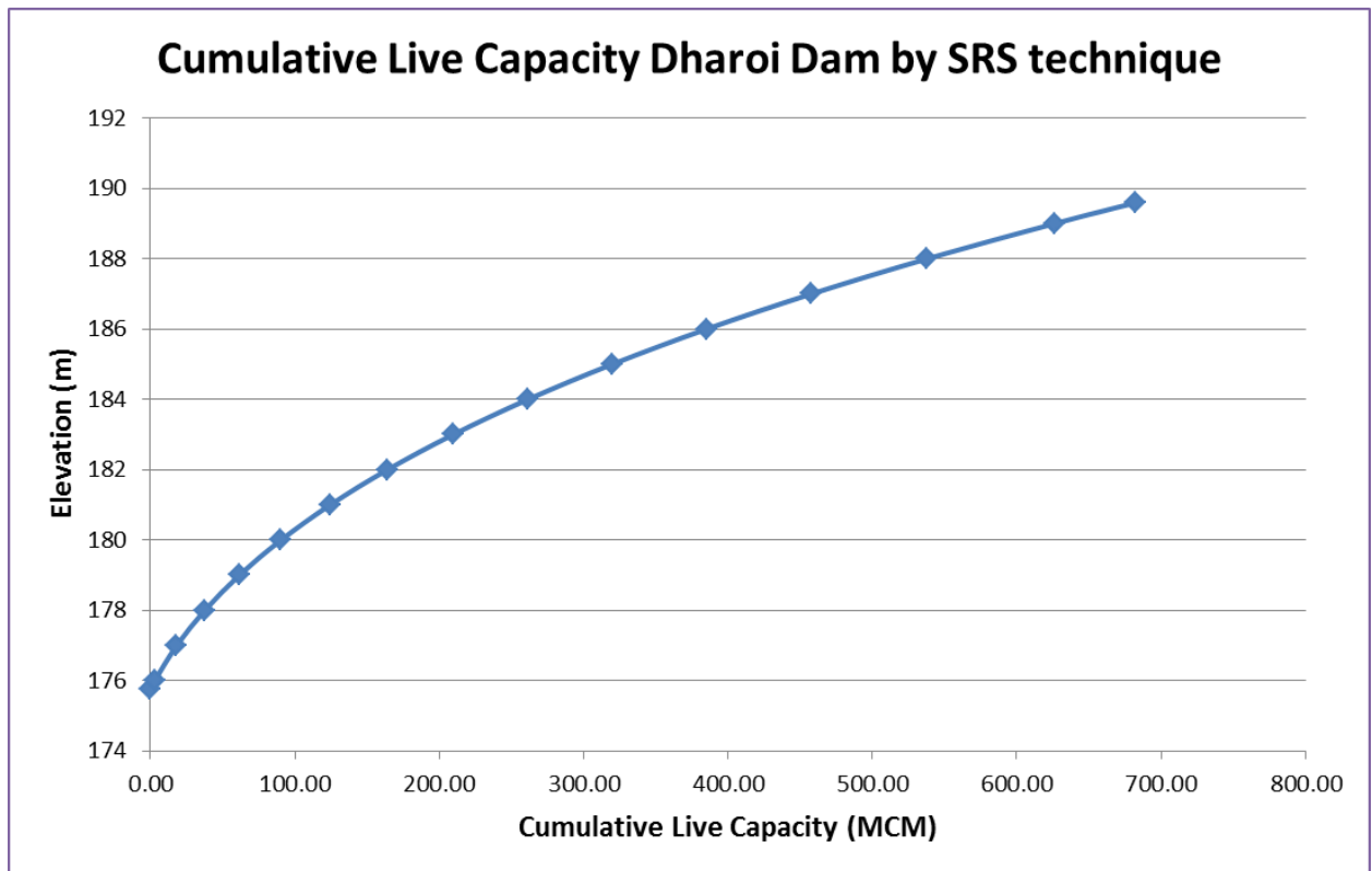
Fig. 9: Modified live capacity - elevation curve (SRS technique)
