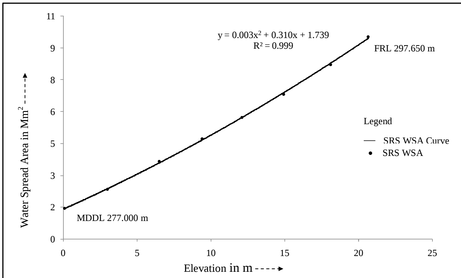
Figure 8 : SRS Elevation-Area curve for Man reservoir, Madhya Pradesh
