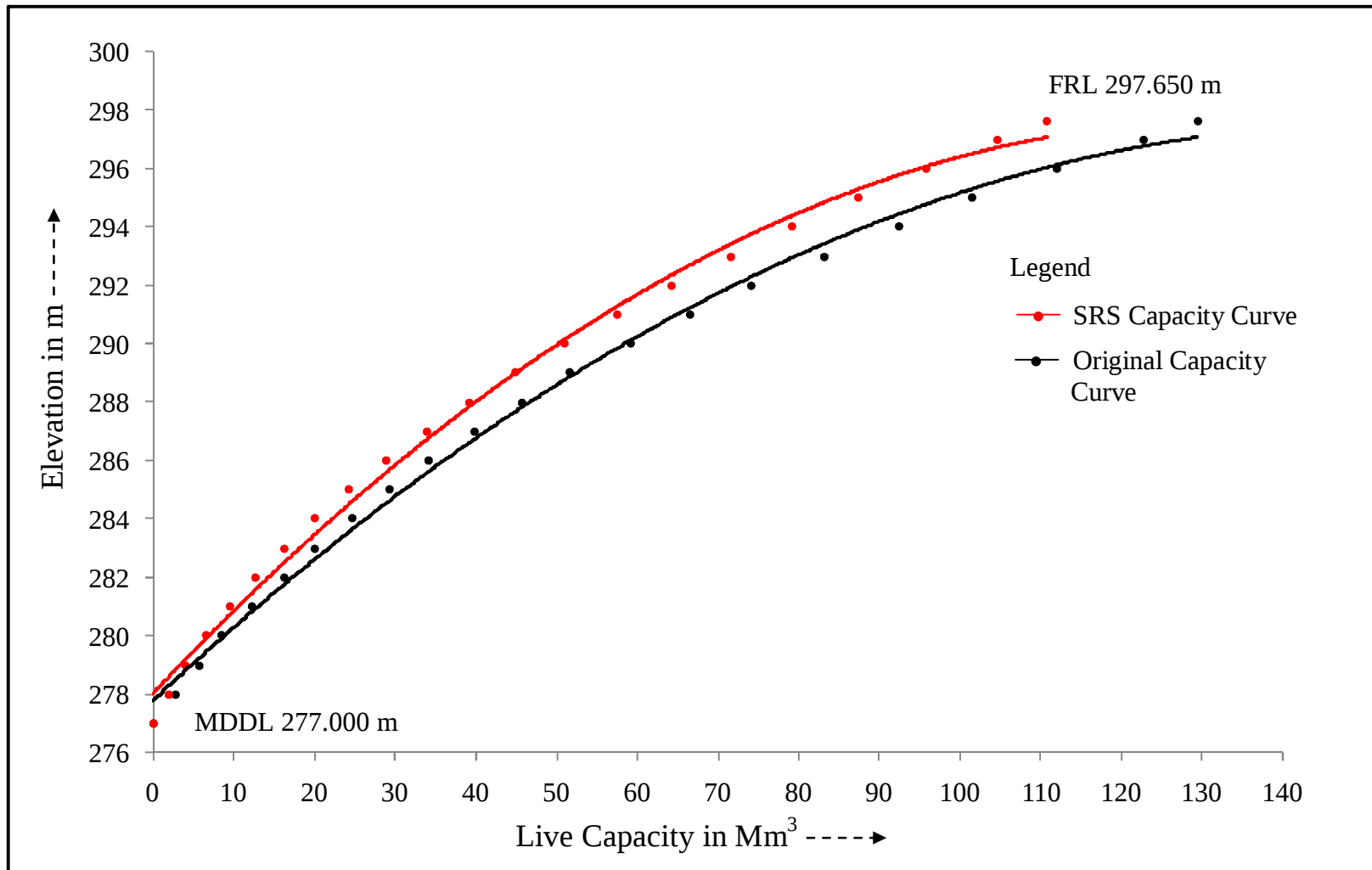
Figure 11 : Elevation - Capacity curve for different years for Man reservoir, Madhya Pradesh
