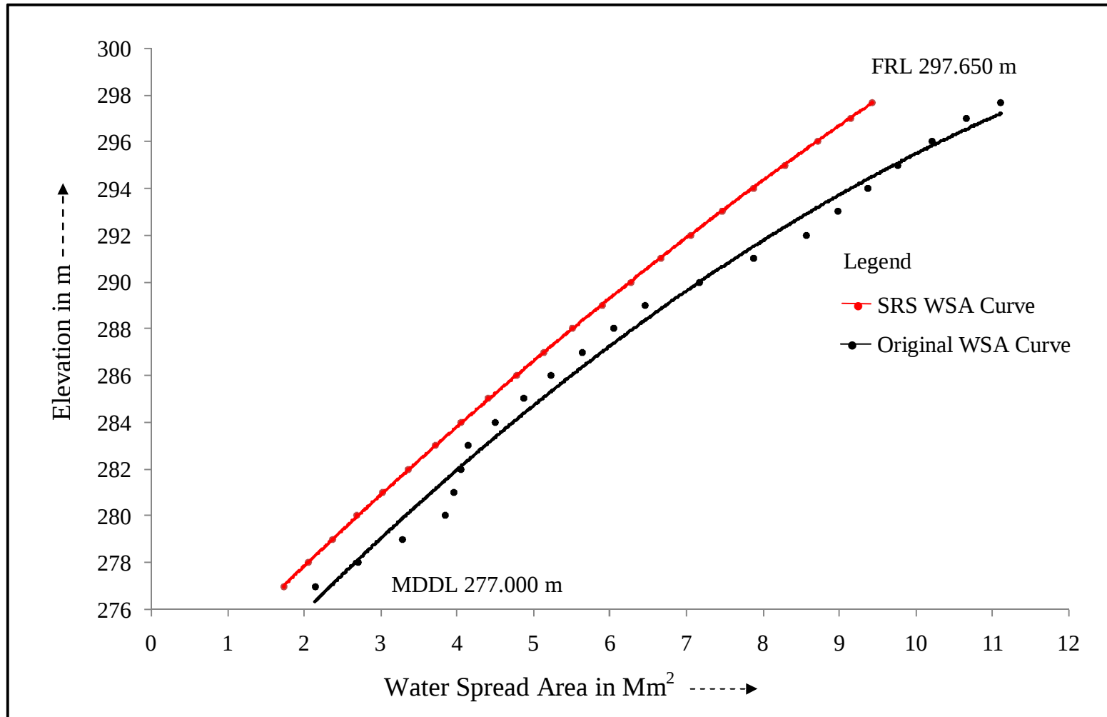
Figure 10 : Elevation - Area curve for different years for Man reservoir, Madhya Pradesh
