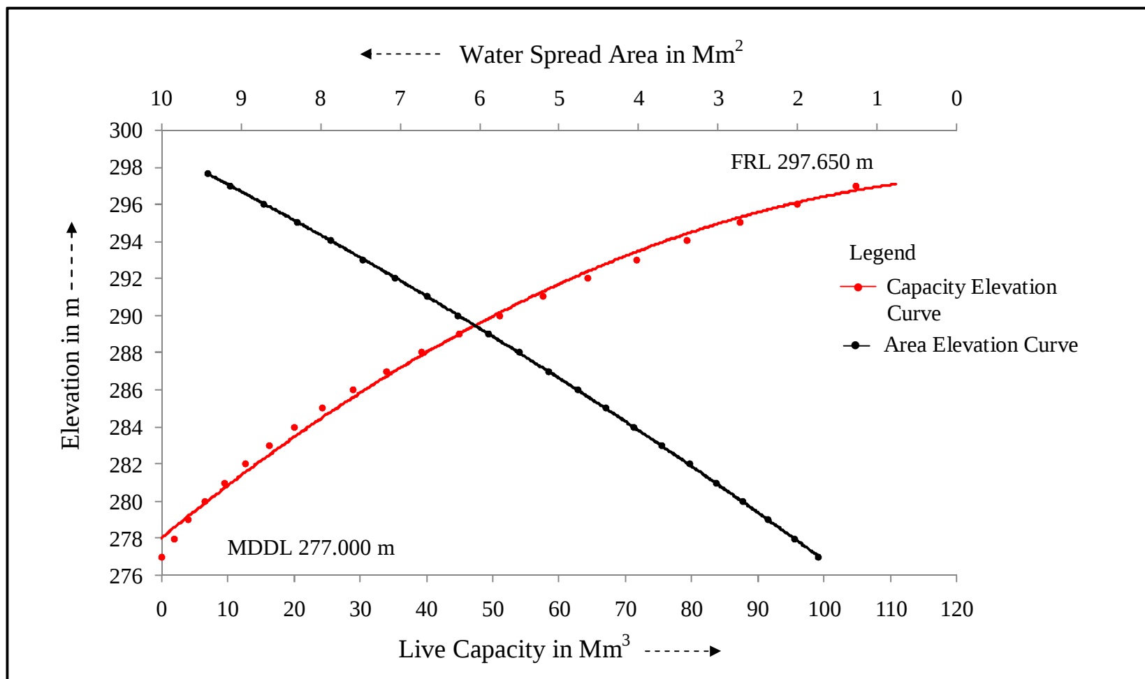
Figure 12 : Modified SRS Elevation - Area - Capacity curve for Man reservoir, Madhya Pradesh
