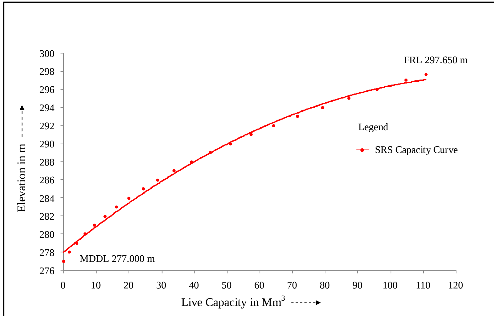
Figure 9 : SRS Elevation-Capacity curve for Man reservoir, Madhya Pradesh
