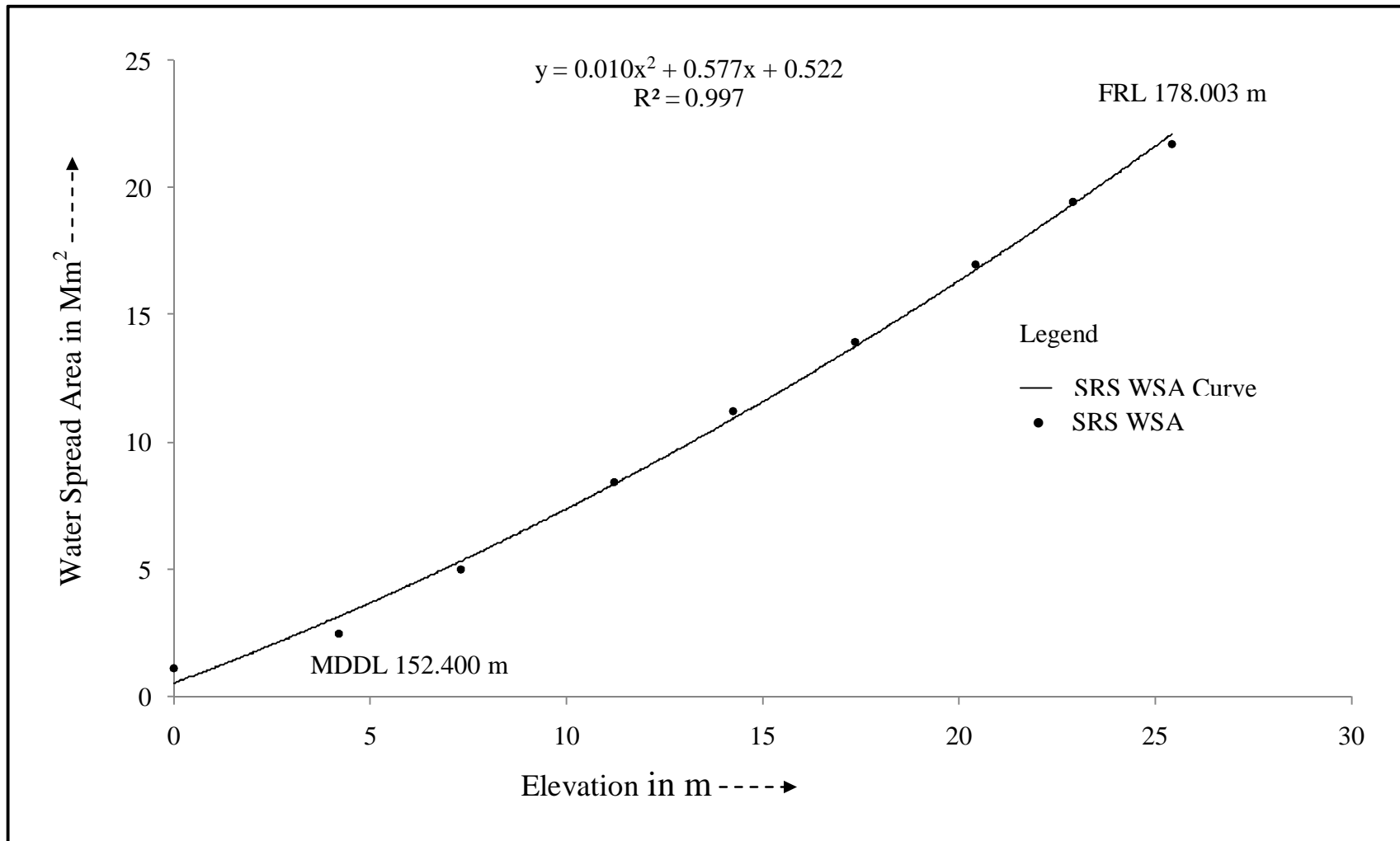
Figure 8 : SRS Elevation-Area curve for Meja reservoir, Uttar Pradesh
