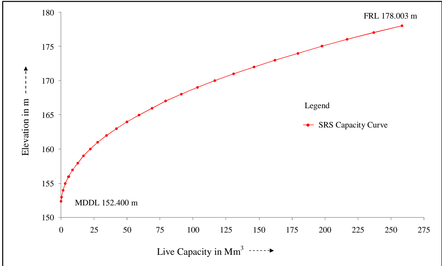
Figure 9 : SRS Elevation-Capacity curve for Meja reservoir, Uttar Pradesh
