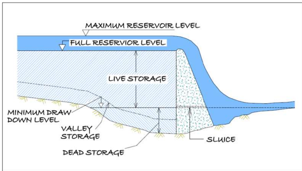
Figure 3 : Conceptual sketch of different levels in a reservoir
