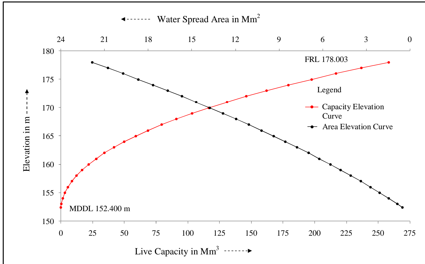
Figure 12 : Modified SRS Elevation - Area - Capacity curve for Meja reservoir, Uttar Pradesh
