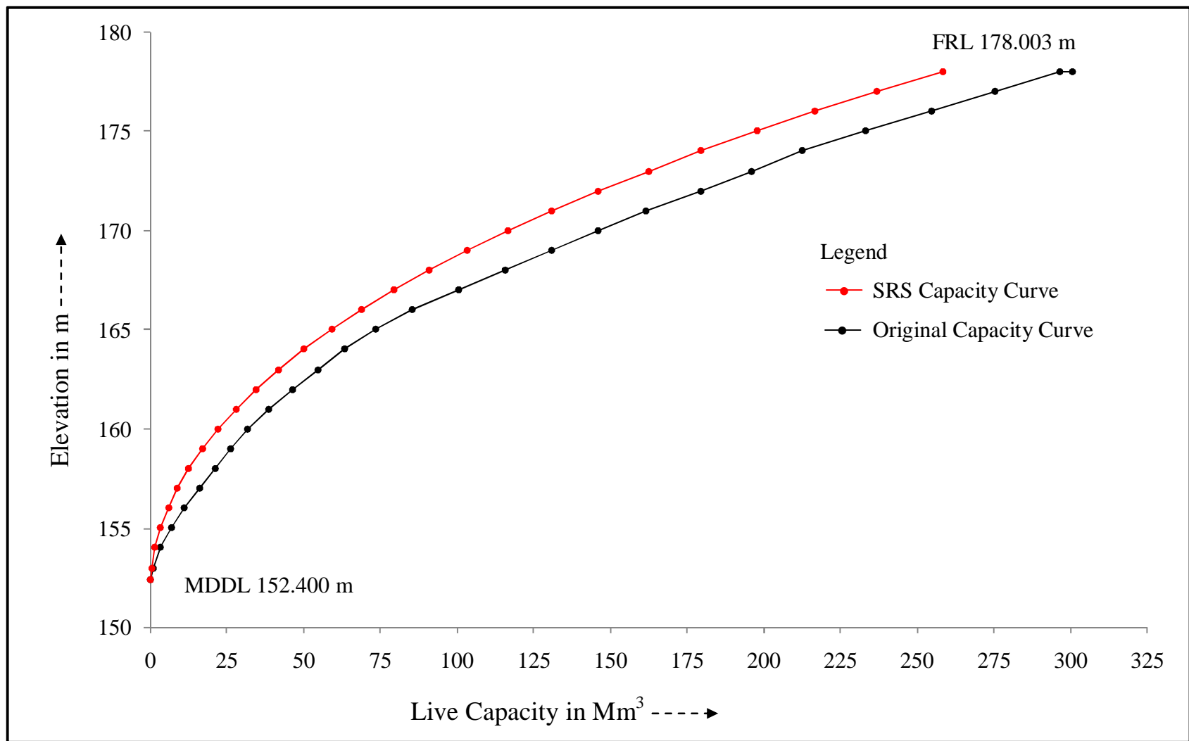
Figure 11 : Elevation - Capacity curve for different years for Meja reservoir, Uttar Pradesh
