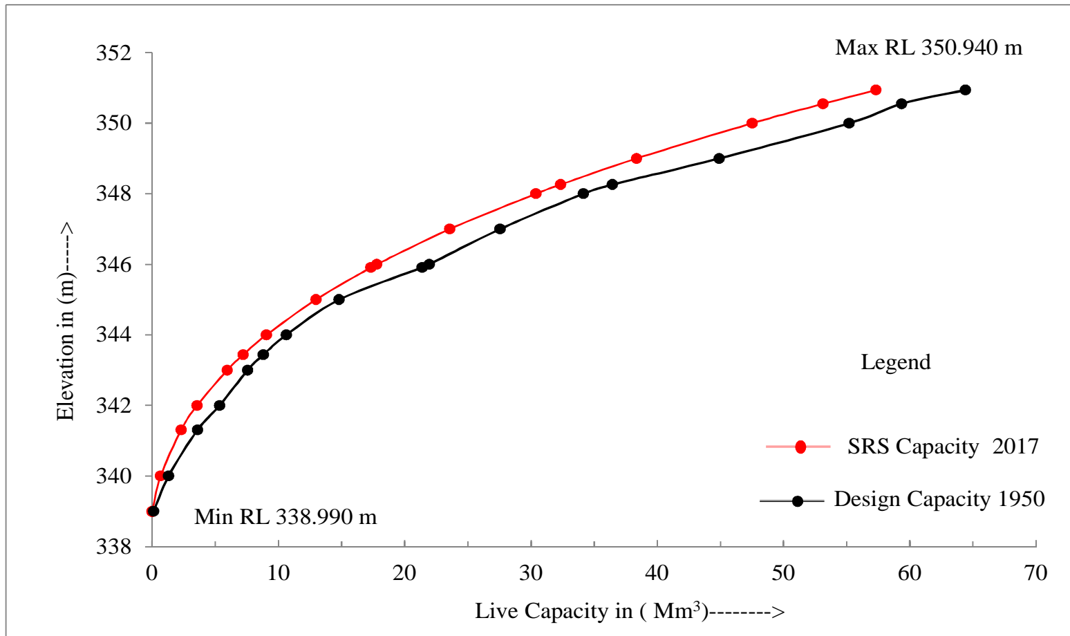
Figure 11 : Elevation - Capacity curve for different years for Nagawa reservoir, Uttar Pradesh
