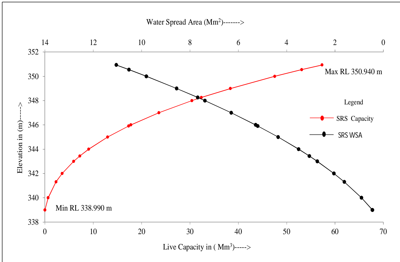
Figure 12 : Modified SRS Elevation- Area- capacity curve for Nagawa reservoir, Uttar Pradesh
