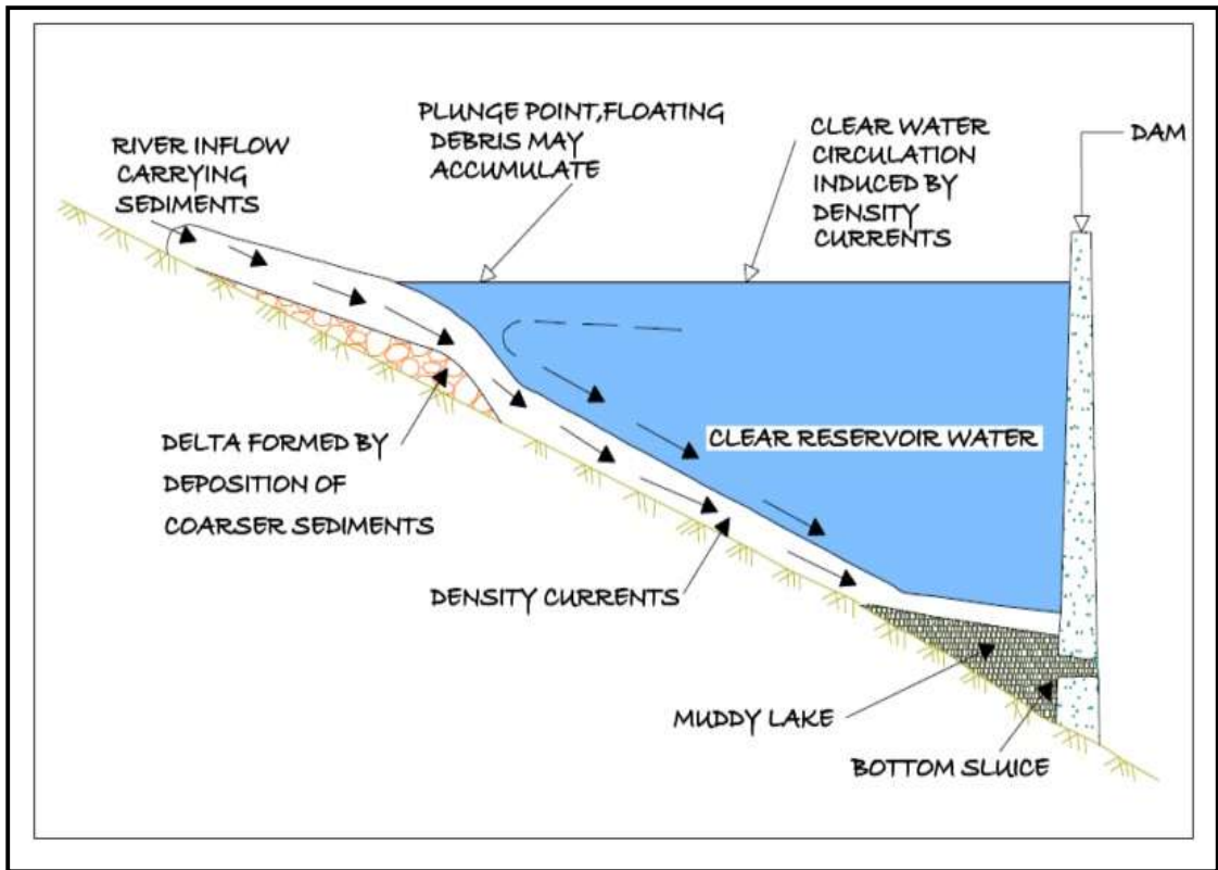
Figure 1: Conceptual sketch of density currents in a reservoir
