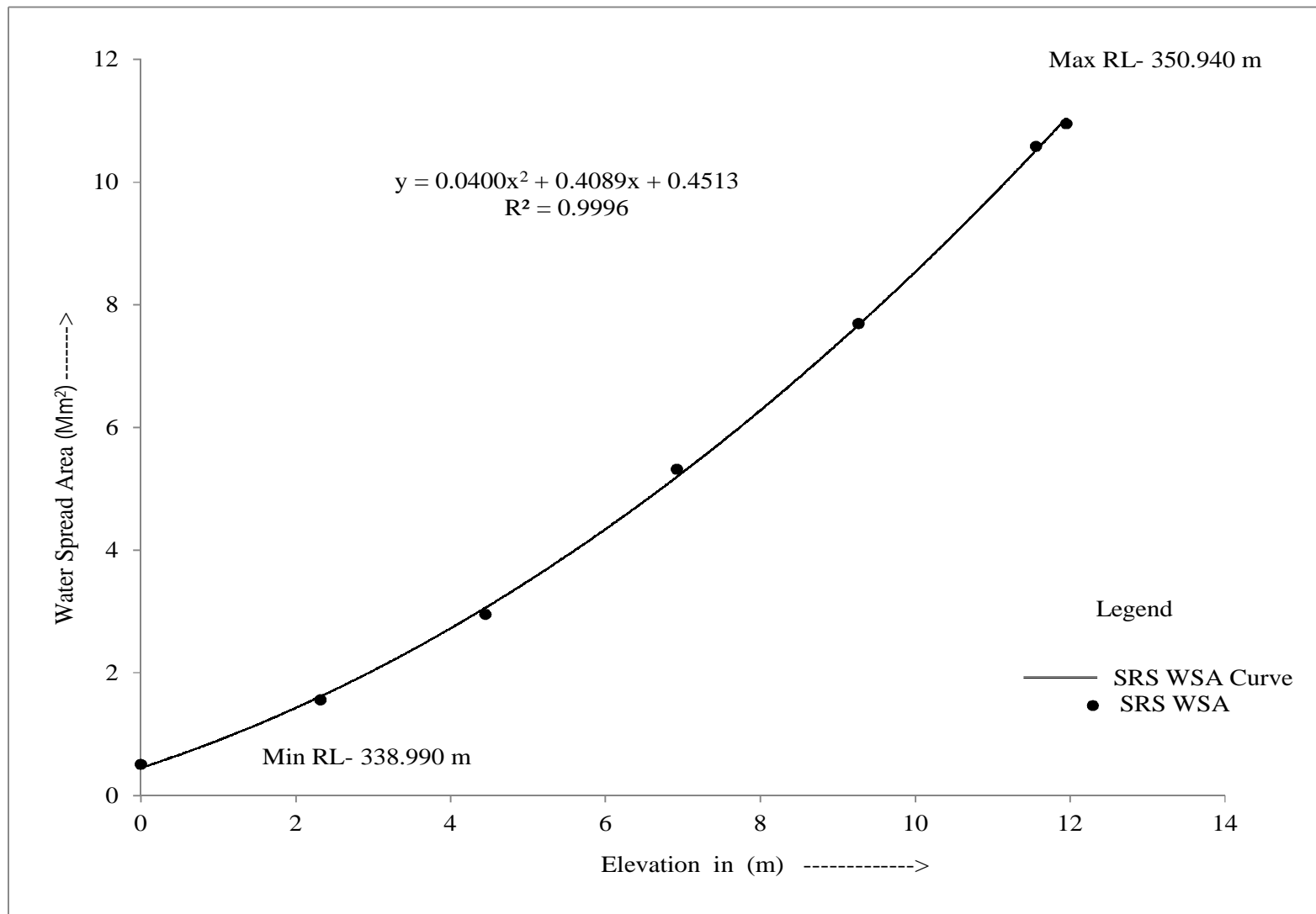
Figure 8 : SRS Elevation-Area curve for Nagawa reservoir, Uttar Pradesh
