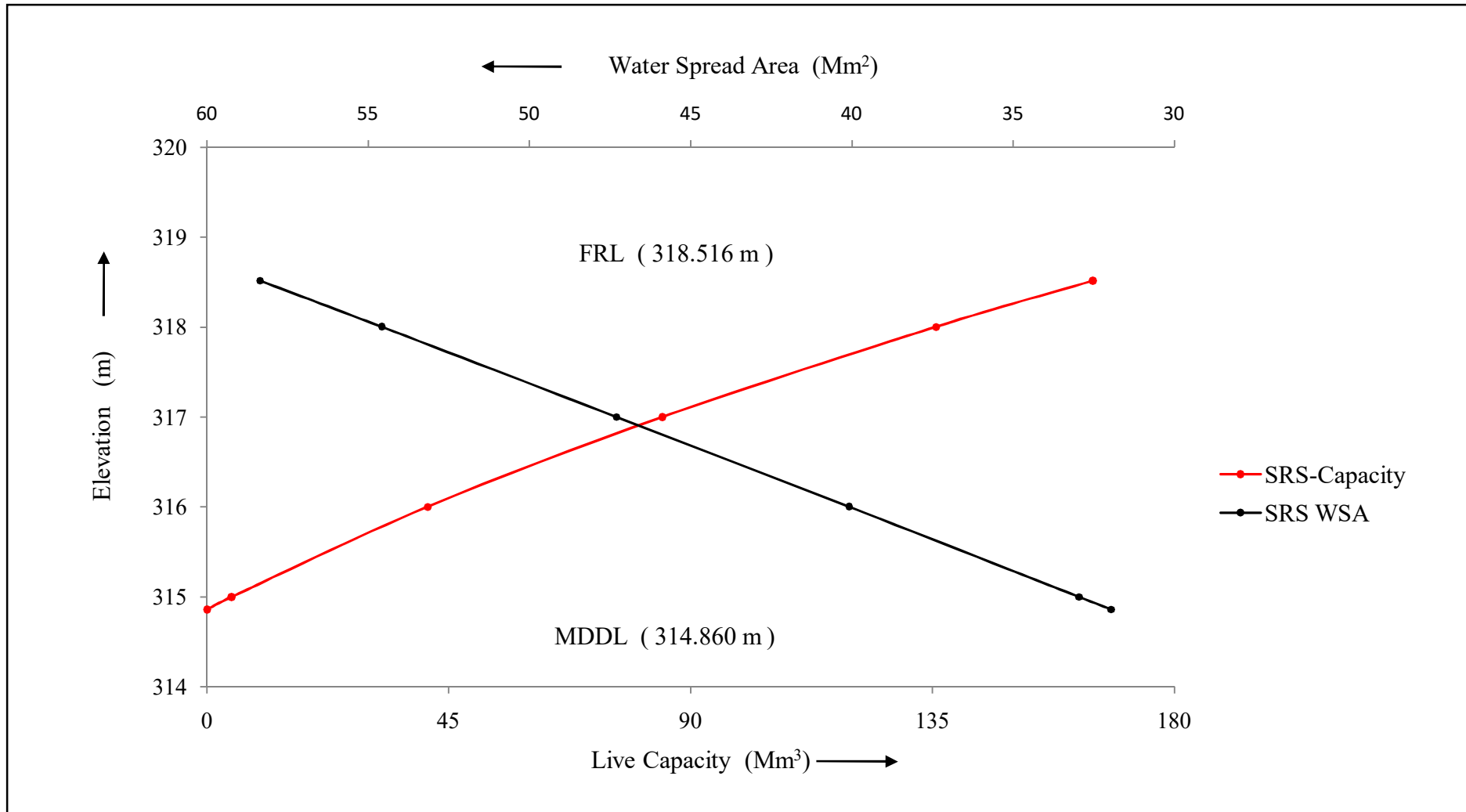
Figure 12 : Modified SRS Elevation-Area-Capacity curve for Priyadarshini Jurala reservoir, Telangana
