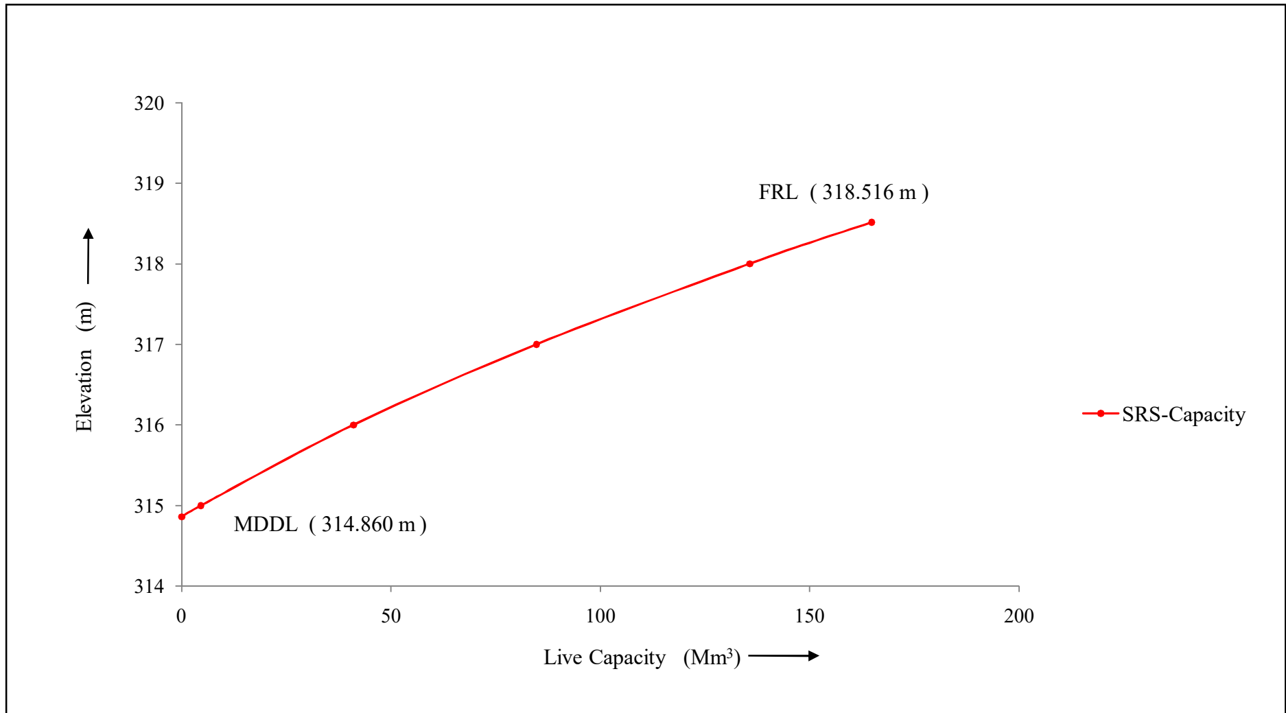
Figure 9 : SRS Elevation-Capacity curve for Priyadarshini Jurala reservoir, Telangana
