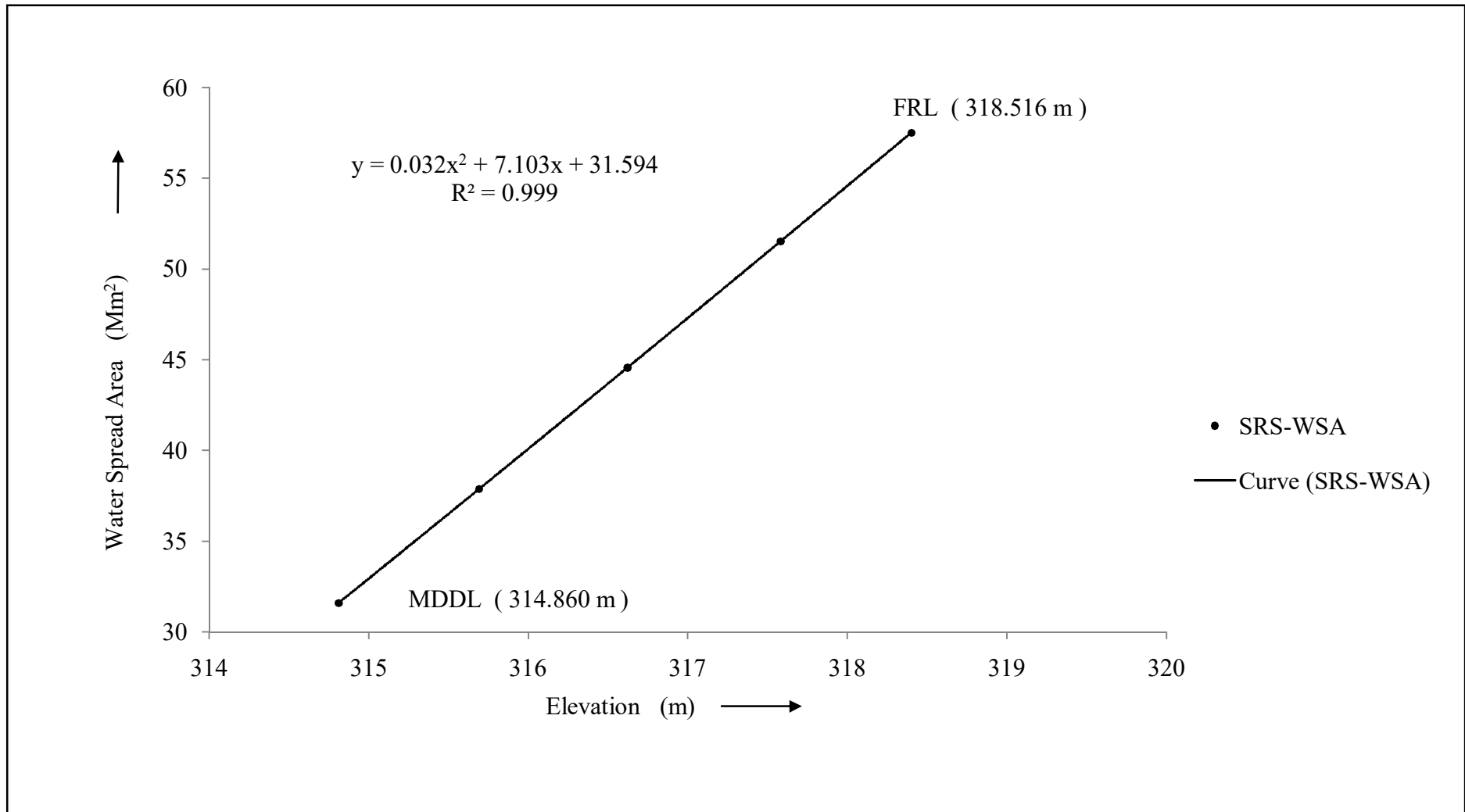
Figure 8 : SRS Elevation-Area curve for Priyadarshini Jurala reservoir, Telangana
