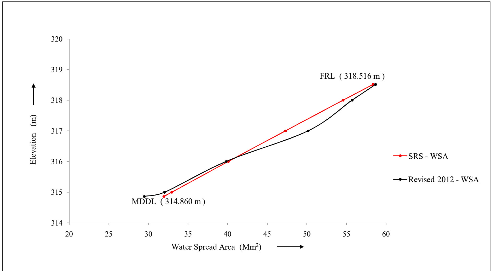
Figure 10 : Elevation-Area curve for different years for Priyadarshini Jurala reservoir, Telangana
