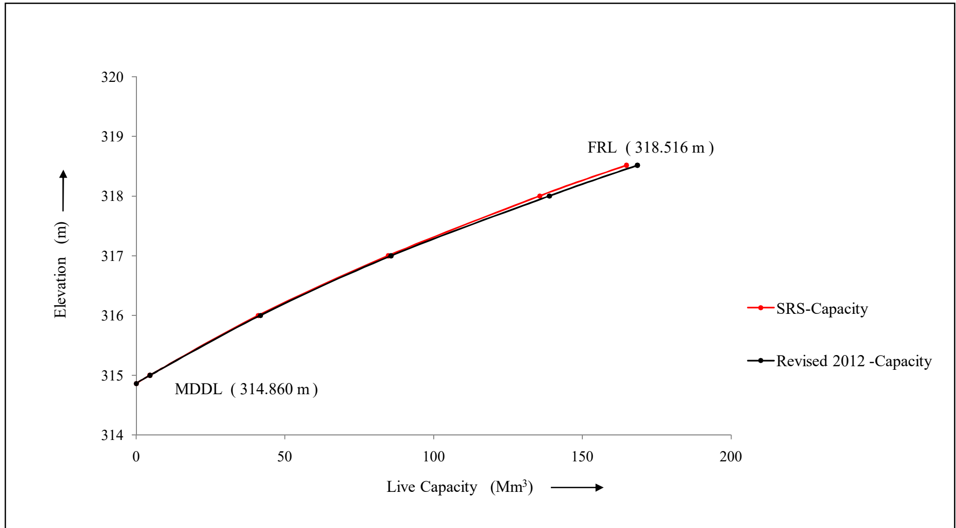
Figure 11 : Elevation-Capacity curve for different years for Priyadarshini Jurala reservoir, Telangana
