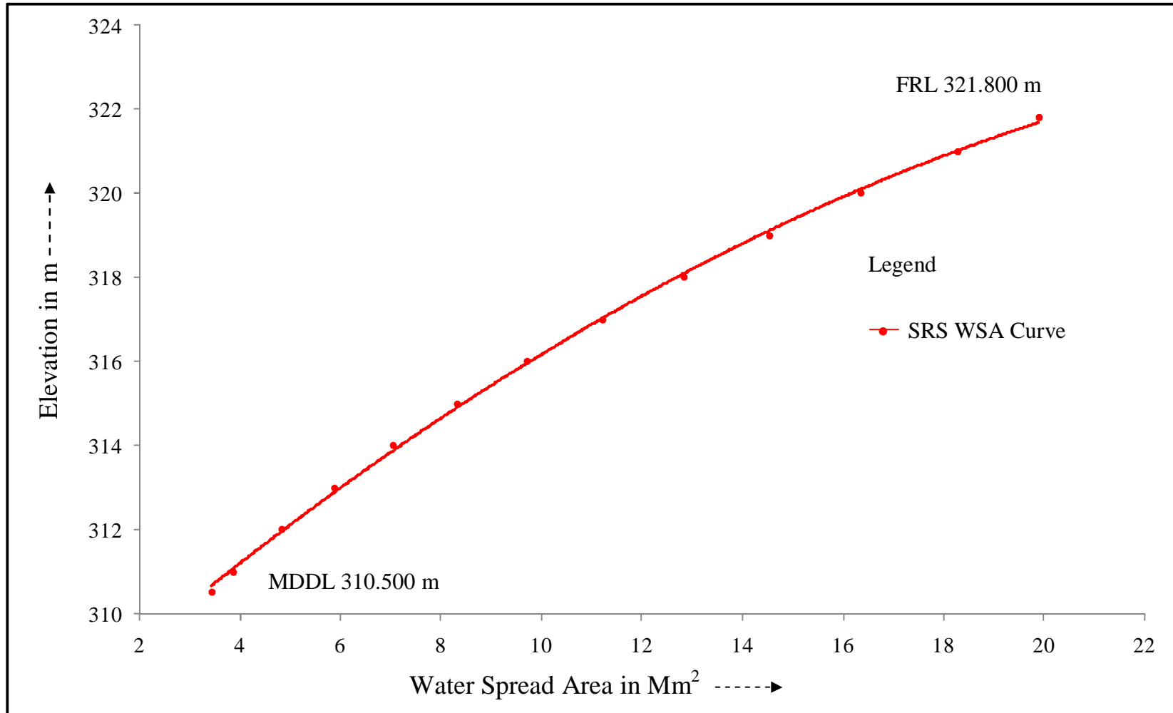
Figure 10 : Elevation - Area curve for different years for Shahzad reservoir, Uttar Pradesh
