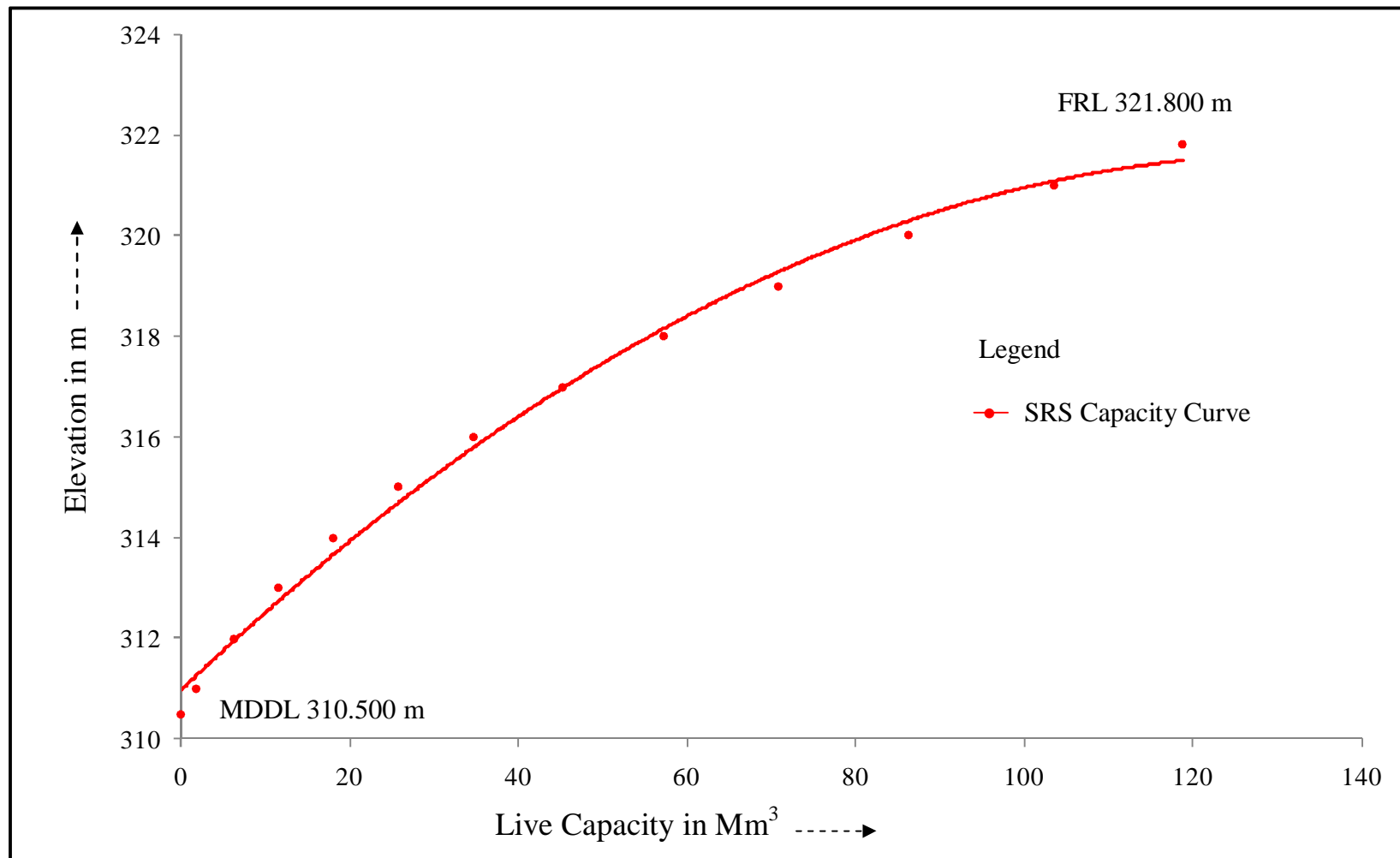
Figure 9 : SRS Elevation-Capacity curve for Shahzad reservoir, Uttar Pradesh
