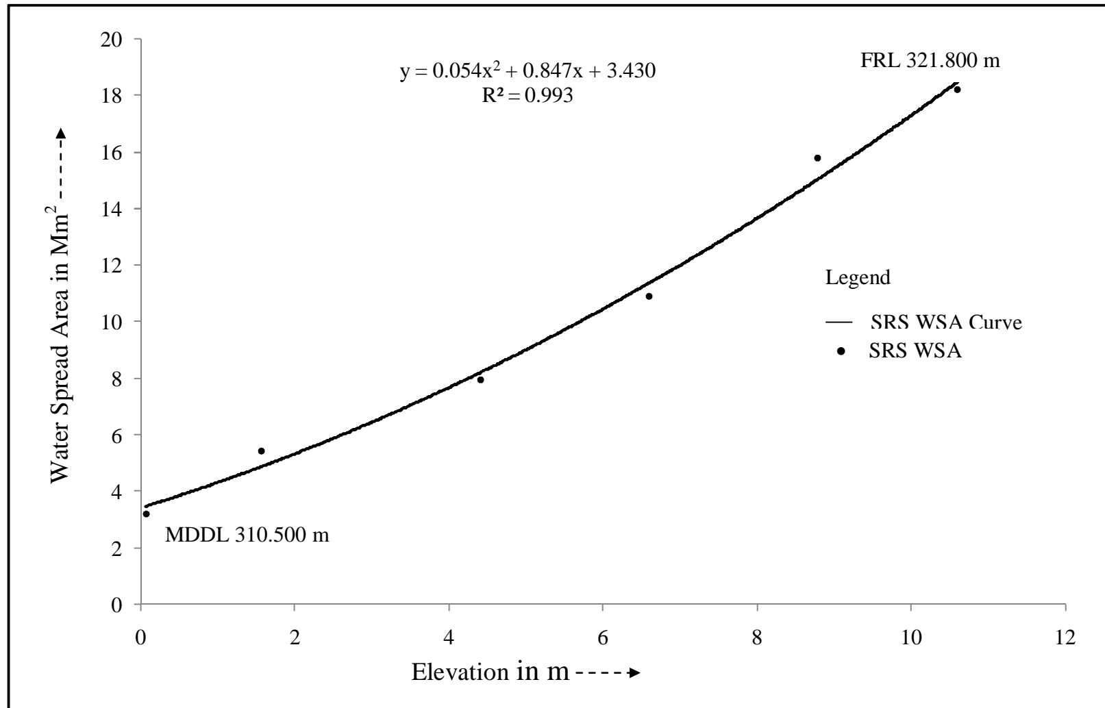
Figure 8 : SRS Elevation-Area curve for Shahzad reservoir, Uttar Pradesh
