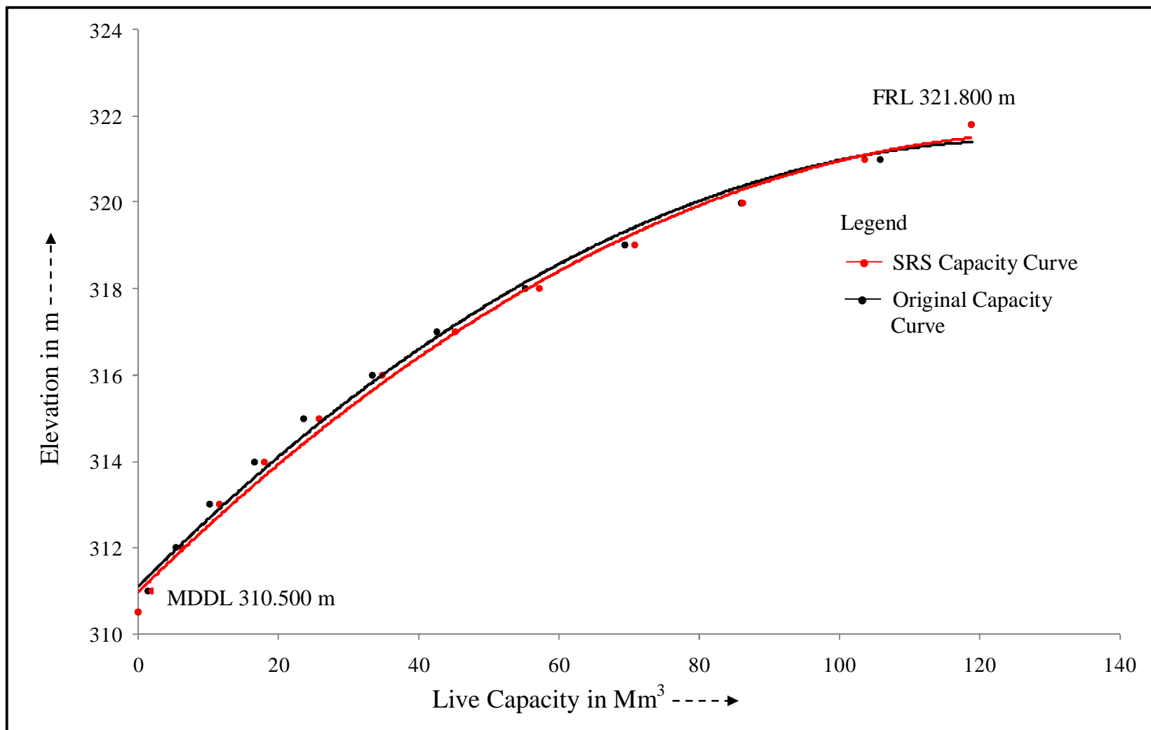
Figure 11 : Elevation - Capacity curve for different years for Shahzad reservoir, Uttar Pradesh
