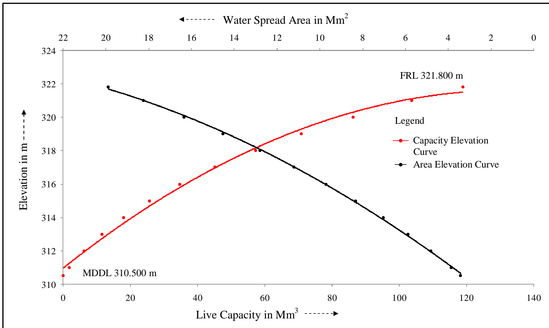
Figure 12 : Modified SRS Elevation - Area - Capacity curve for Shahzad reservoir, Uttar Pradesh
