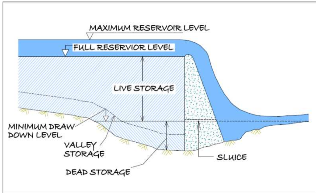
Figure 3 : Conceptual sketch of different levels in a reservoir
