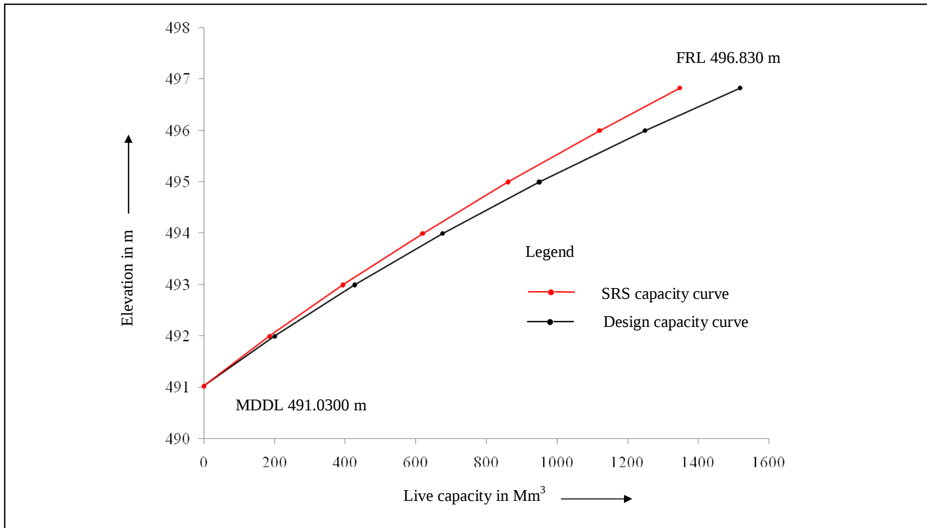
Figure 11 : Elevation- Capacity curve for different years for Ujjani reservoir, Maharashtra
