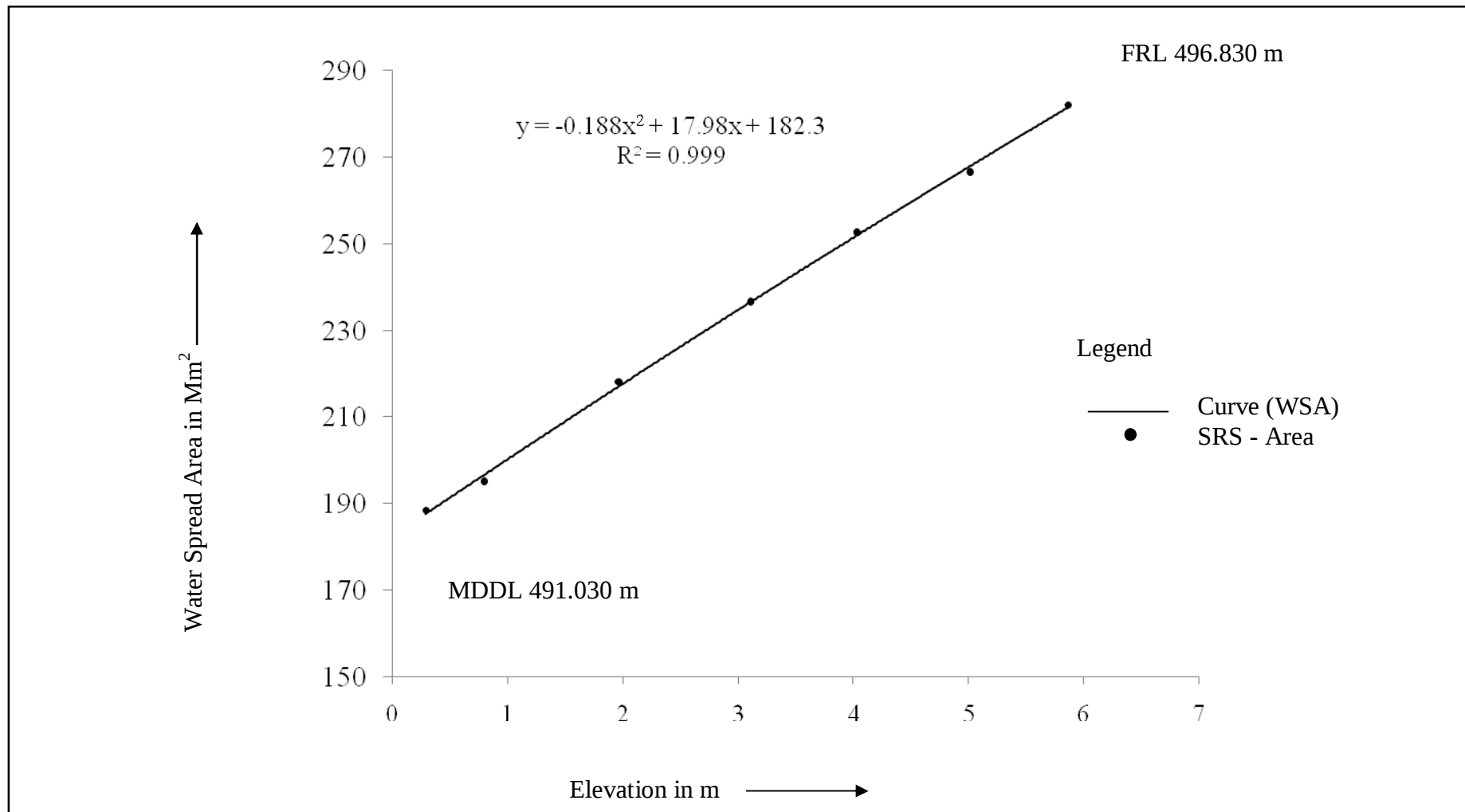
Figure 8 : SRS Elevation-Area curve for Ujjani reservoir, Maharashtra
