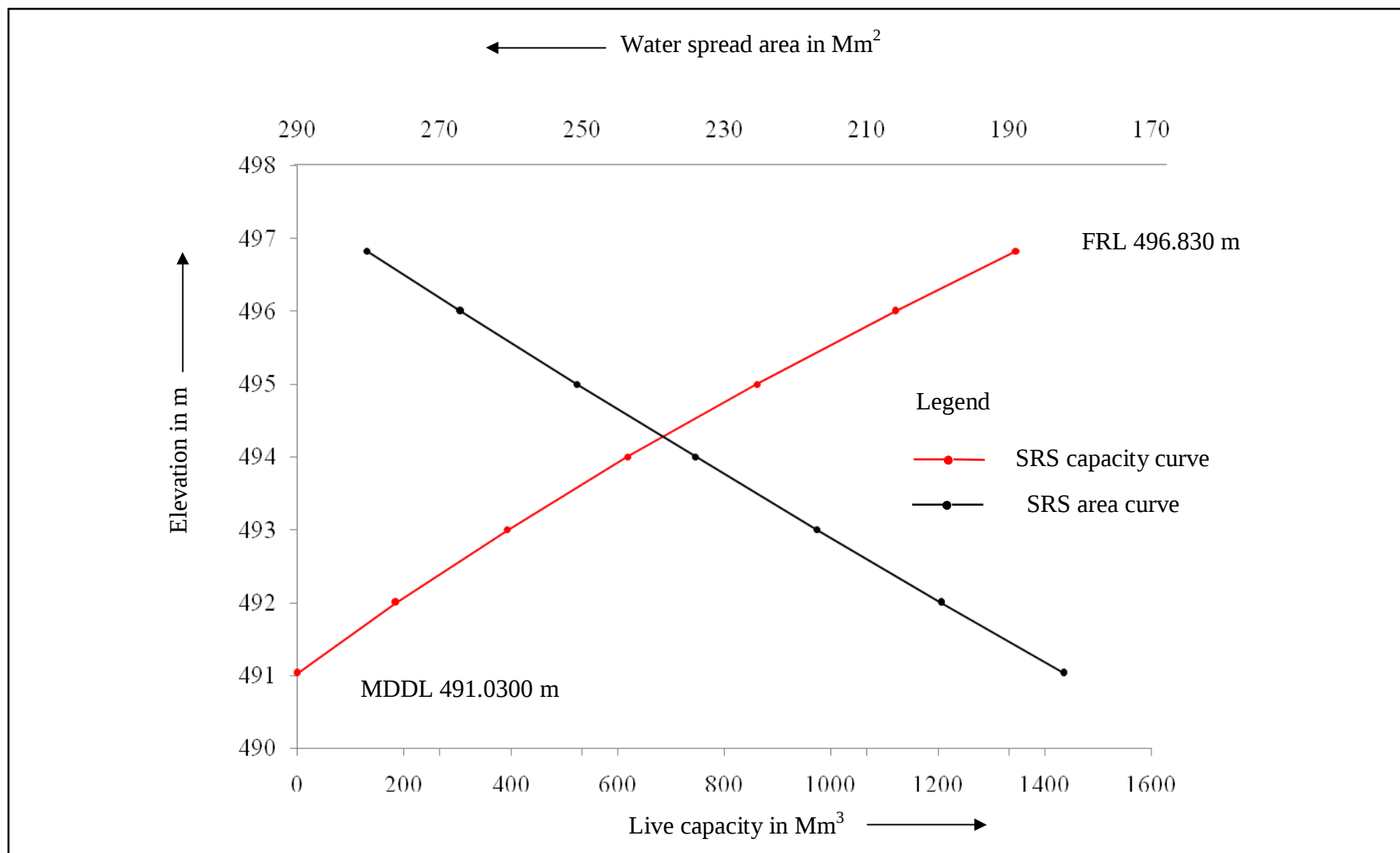
Figure 12 : Modified SRS Elevation - Area- Capacity curve for Ujjani reservoir, Maharashtra
