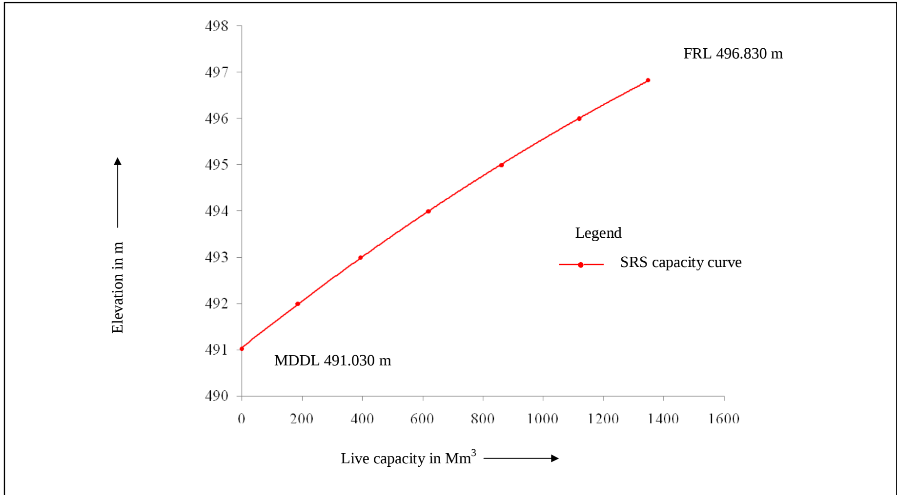
Figure 9 : SRS Elevation-Capacity curve for Ujjani reservoir, Maharashtra
