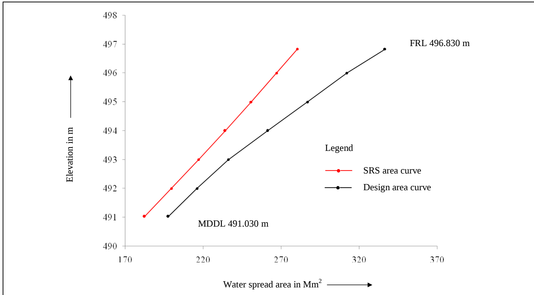
Figure 10 : Elevation - Area curve for different years for Ujjani reservoir, Maharashtra
