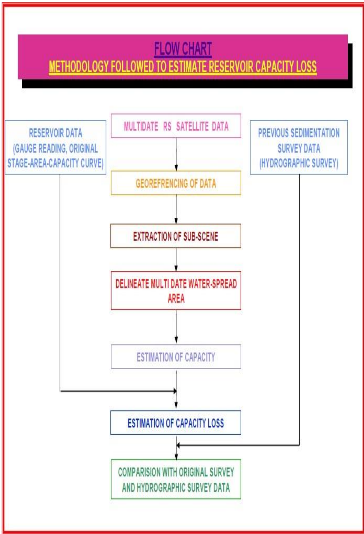
Fig 5 : Flow chart showing methodology followed to estimate reservoir capacity loss
