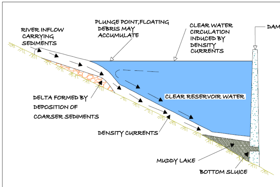
Fig. 1: Conceptual sketch of density currents in a reservoir
