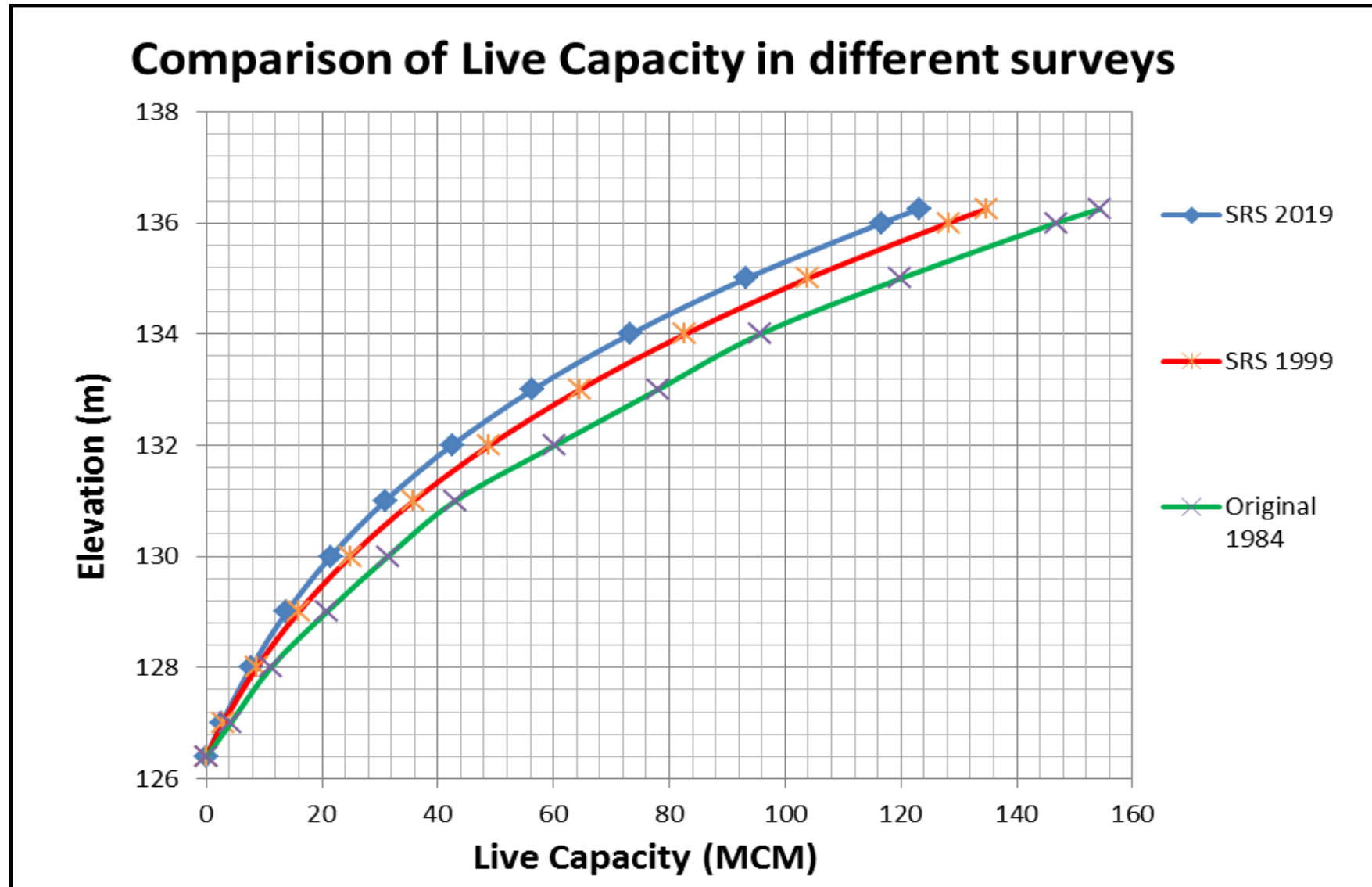
Fig. 11: Comparison of Elevation-Live Storage Capacity Curves in various survey years
