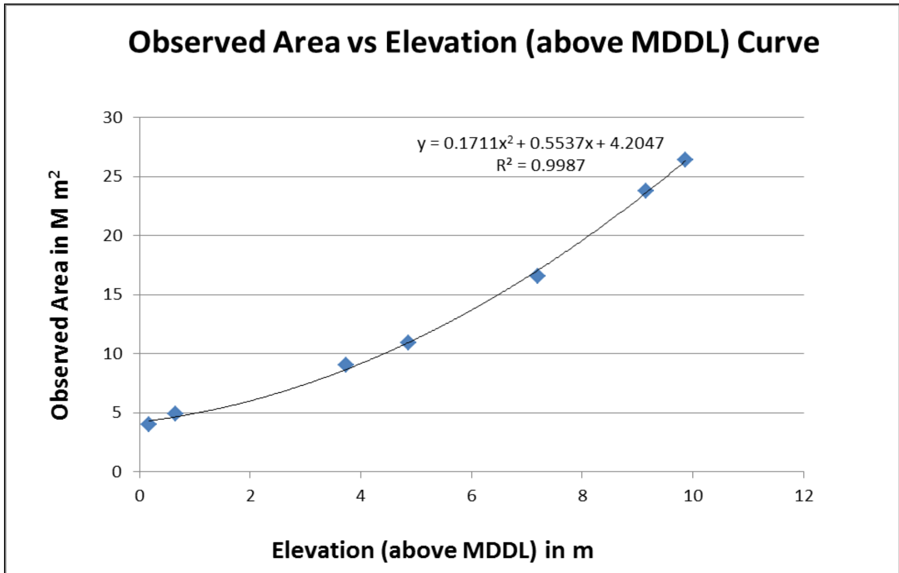
Fig. 8: Elevation vs observed water spread Area of Watrak reservoir
