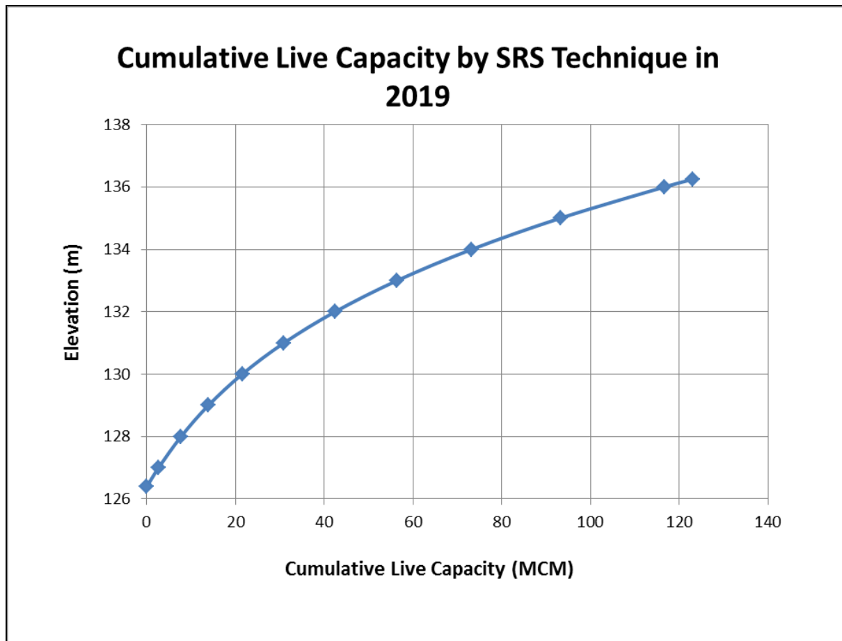
Fig. 9: Modified Live capacity - Elevation curve (SRS technique 2019)
