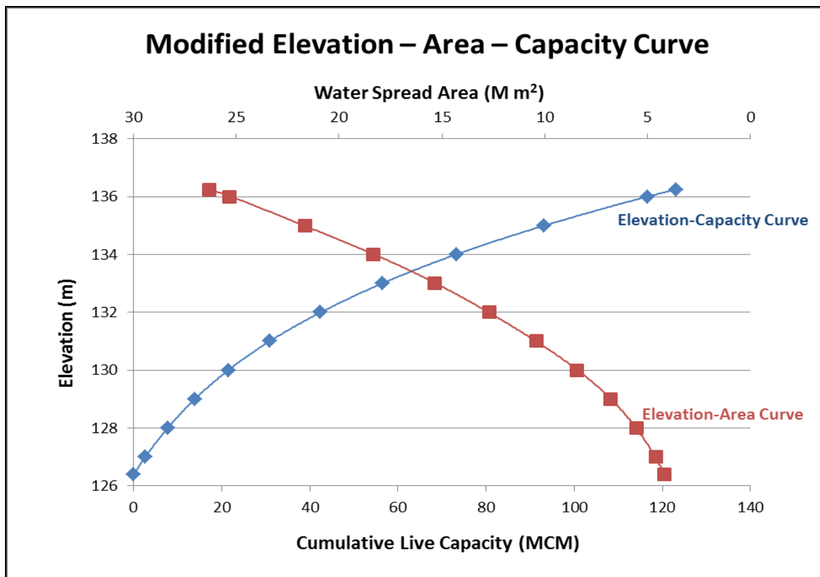
Fig. 10: Modified Elevation – Area – Capacity Curve (SRS technique 2019)
